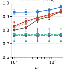
Kendall \tau(\hat{s}, s_0)
