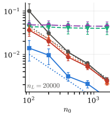
excess human risk
