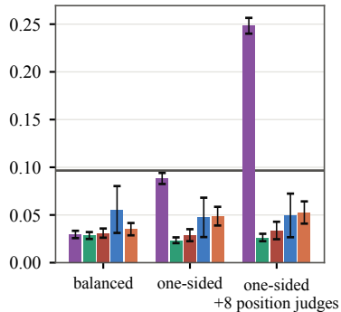
(b) MT-Bench, n_H=80
