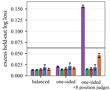
(a) Chatbot Arena, n_H=300
