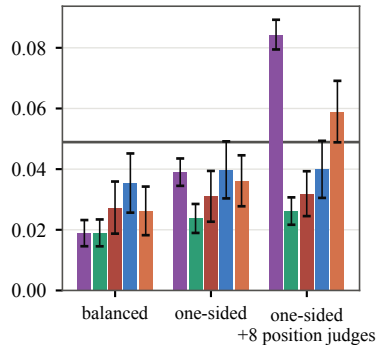
(c) PandaLM, n_H=60
