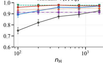
Kendall \tau(\hat{S}, s_0)
