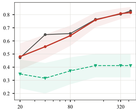
PandaLM, n_L = 100 Kendall's \tau , held-out ranking
