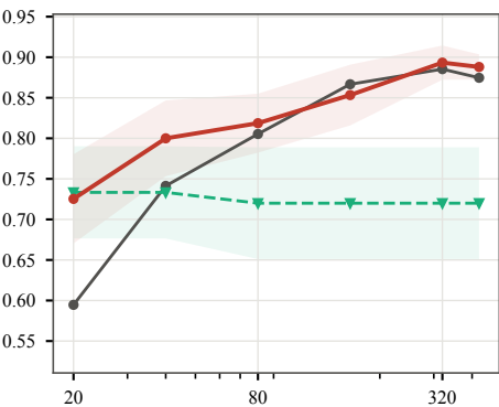
MT-Bench, n_L = 160 Kendall's \tau , held-out ranking
