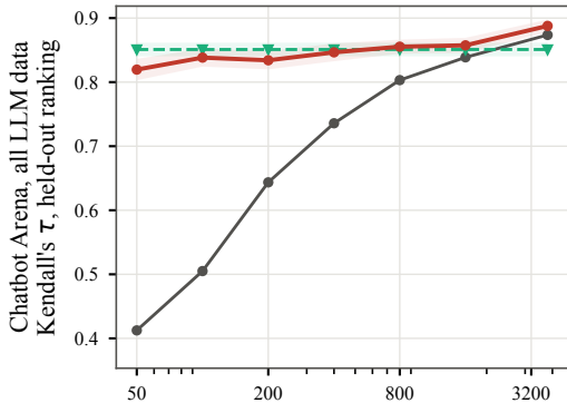
small6 (36.5B)
