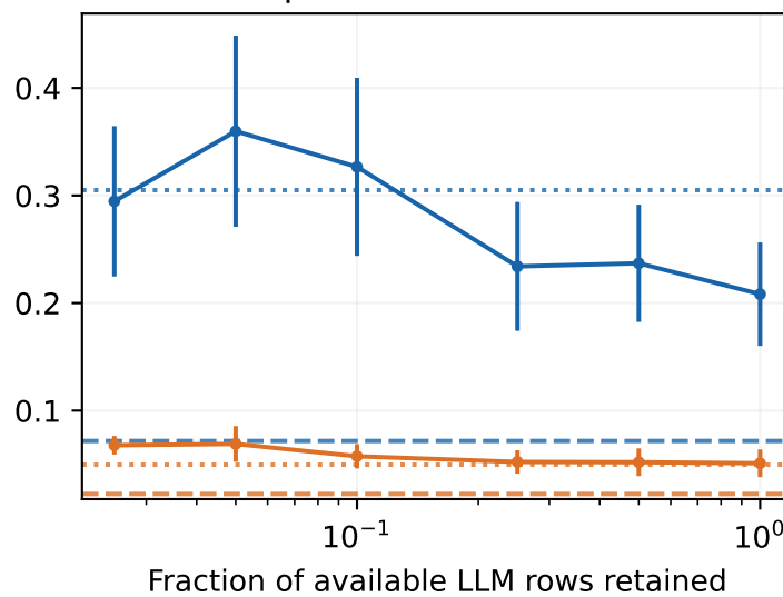
pandalm / small6
