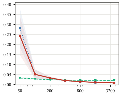
small6 (36.5B)
