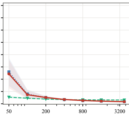
large6 (203B)
