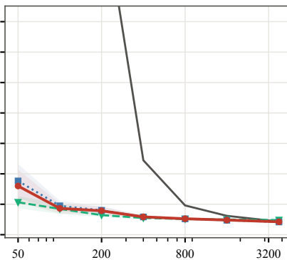
large6 (203B)
