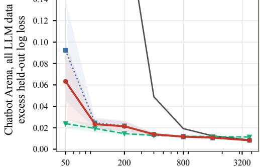
small6 (36.5B)
