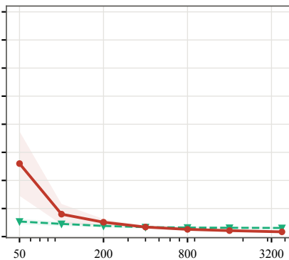
large6 (203B)
