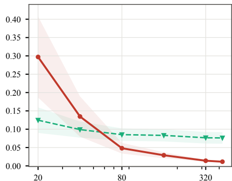
MT-Bench, n_L = 160 excess held-out log loss
