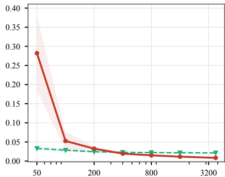
small6 (36.5B)
