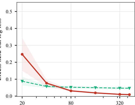
PandaLM, n_L = 100 excess held-out log loss
