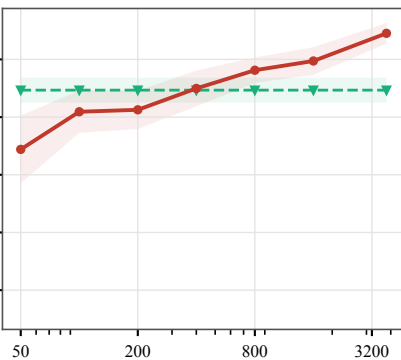
large6 (203B)
