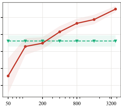
small6 (36.5B)
