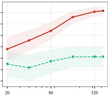
PandaLM, n_L = 100 Kendall's \tau , held-out ranking
