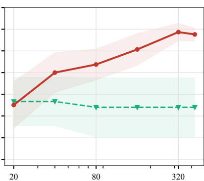
MT-Bench, n_L = 160 Kendall's \tau , held-out ranking
