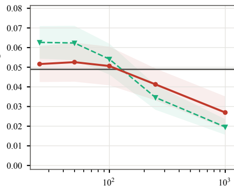
PandaLM, n_H = 60 excess held-out log loss
