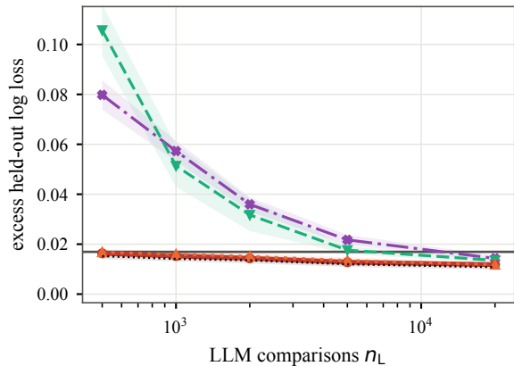
Chatbot Arena, 5 biased judges, n_H=1000
