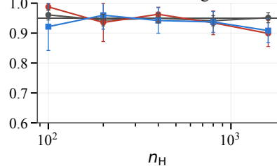
95% CI coverage
