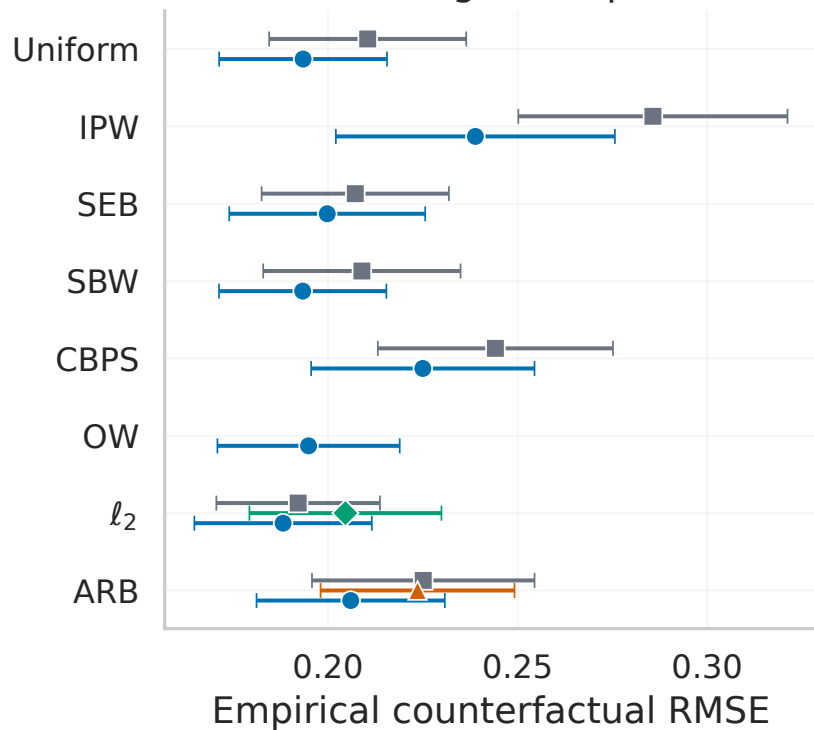
Strong overlap
