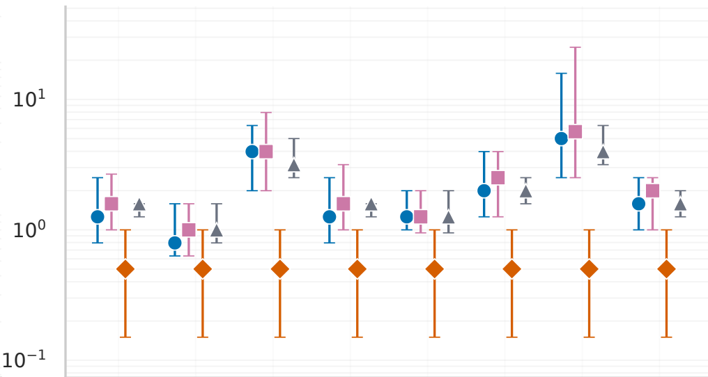
Intermediate weak overlap
