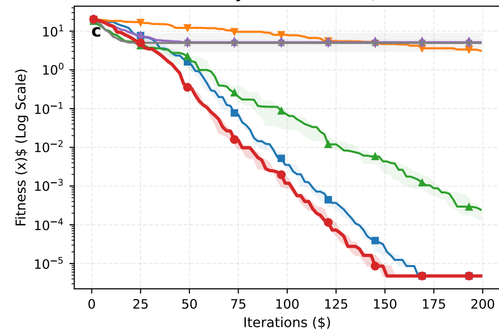
Ackley Function (=10$)
