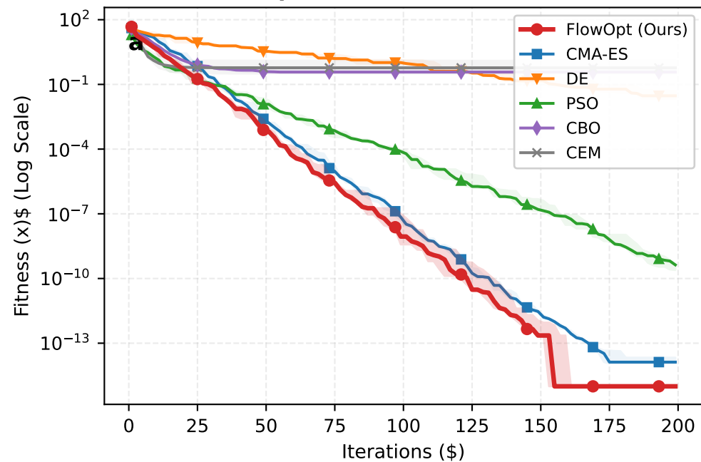
Ackley Function (=10$)
