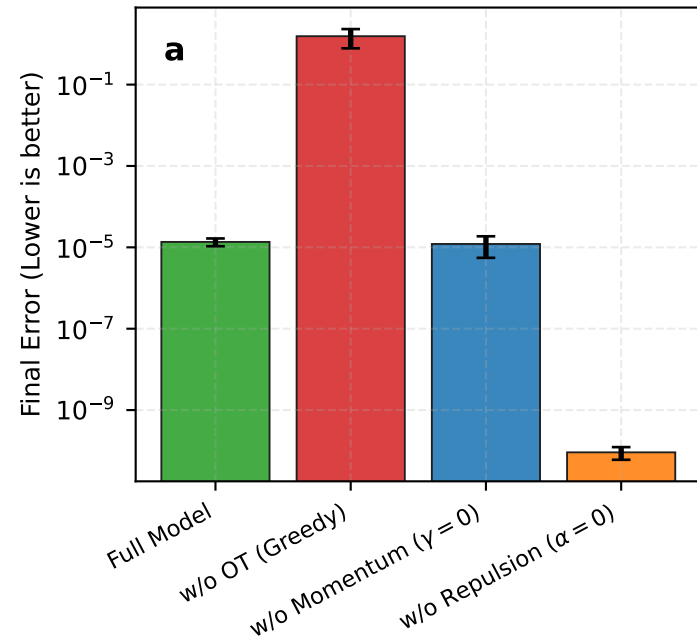
Sphere Function
