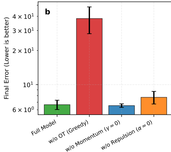
Rosenbrock Function
