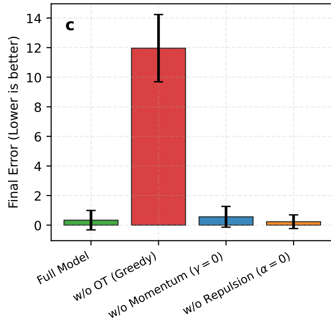
Ackley Function
