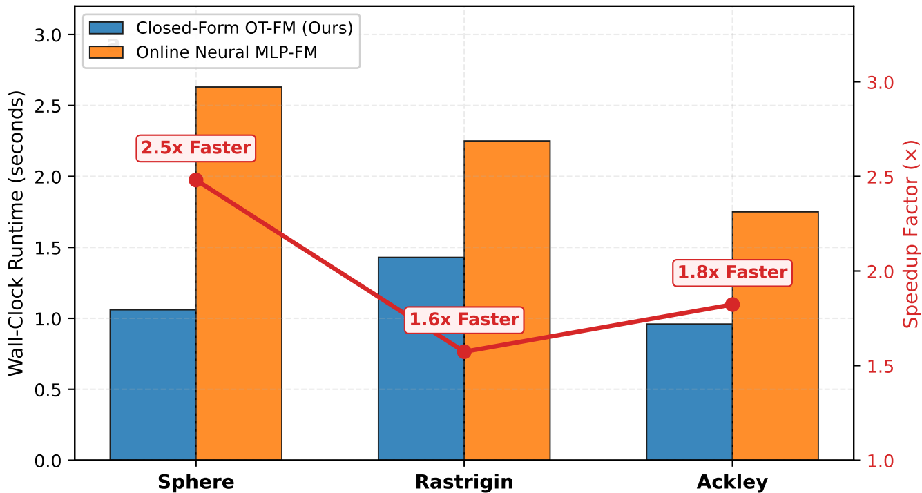
Computational Latency: Closed-Form vs. Online Neural Vector Field
