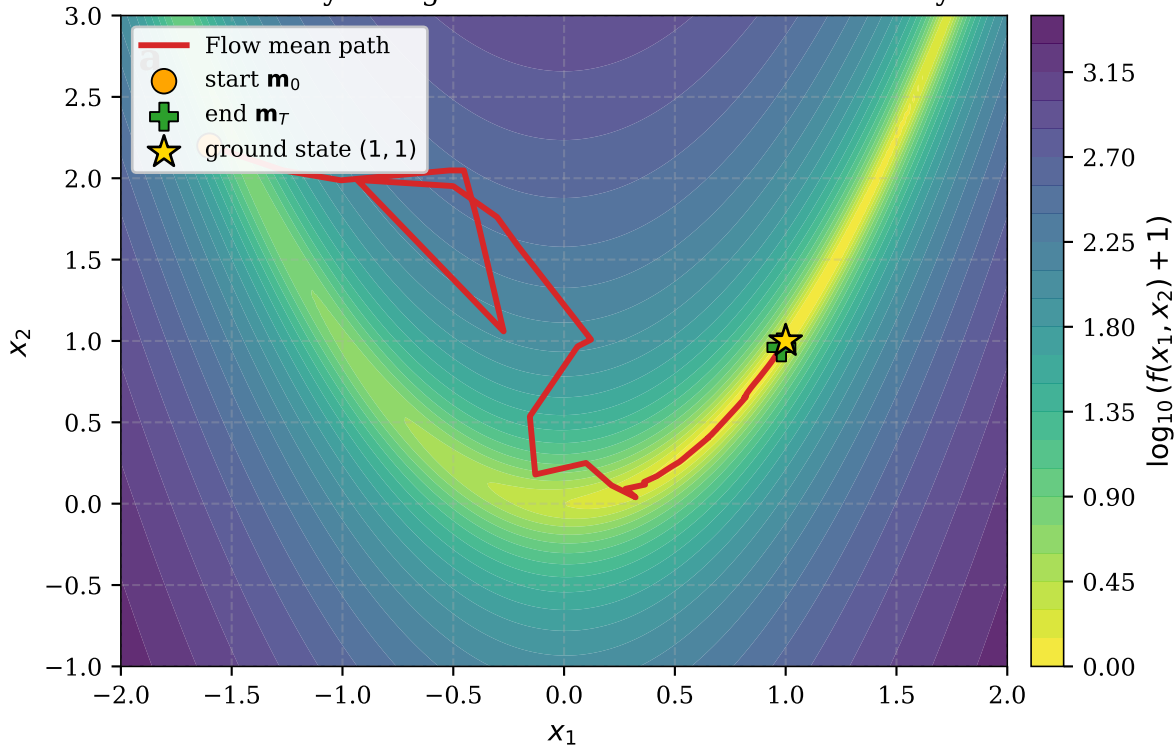
Probability-flow geodesics on the Rosenbrock valley
