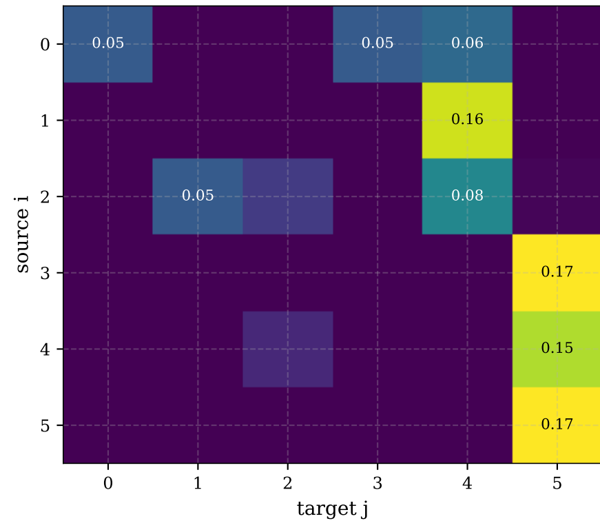
Coupling \Pi^* (Sinkhorn)
