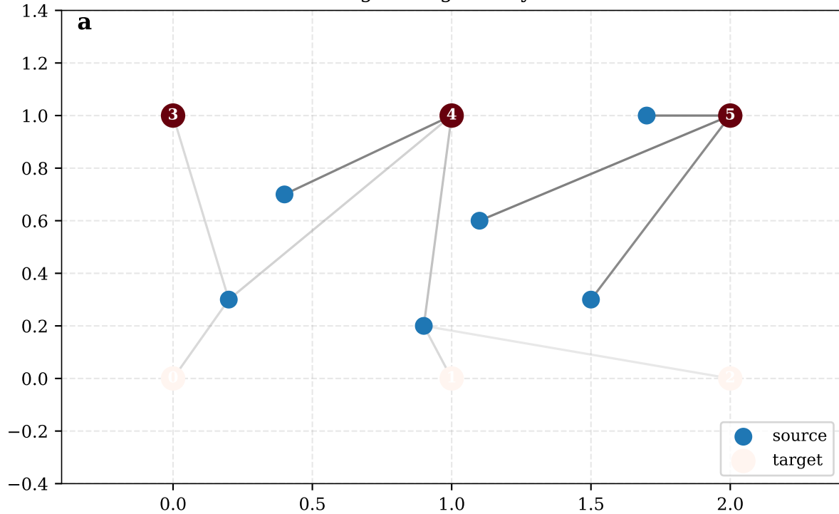
edges weighted by \Pi^*
