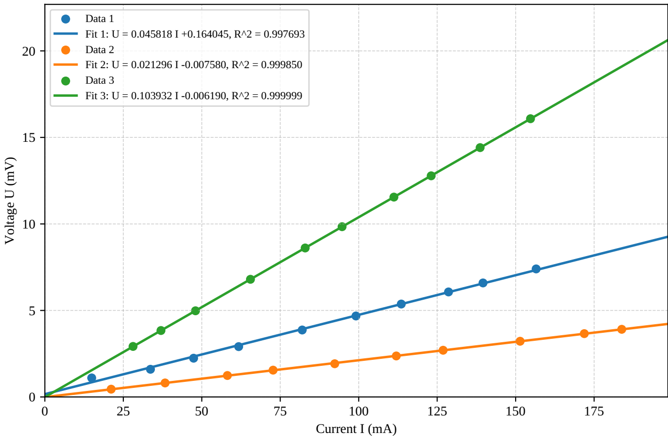
Linear Least-Squares Fitting of U-I Data
