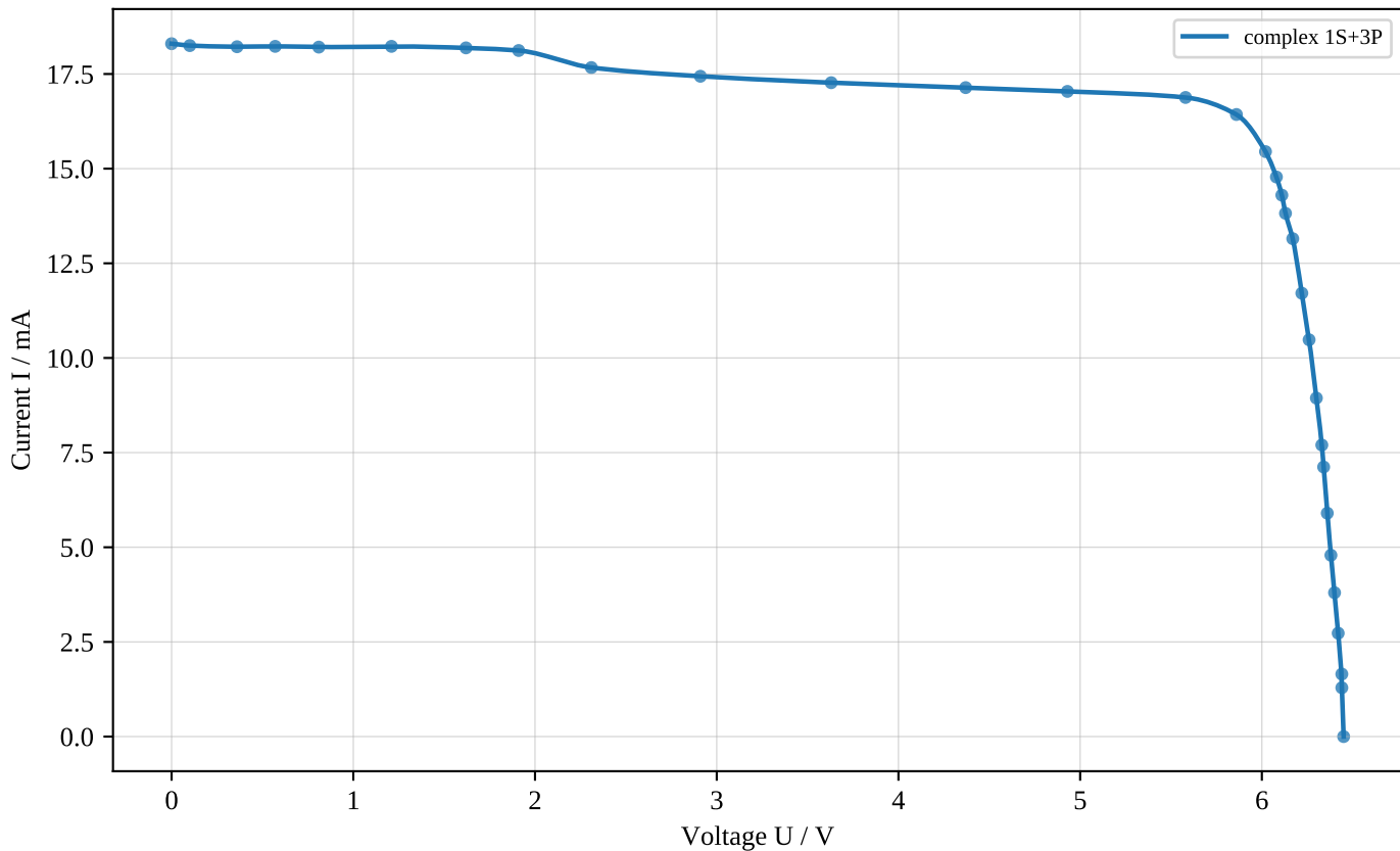
I-V curve: complex 1S+3P
