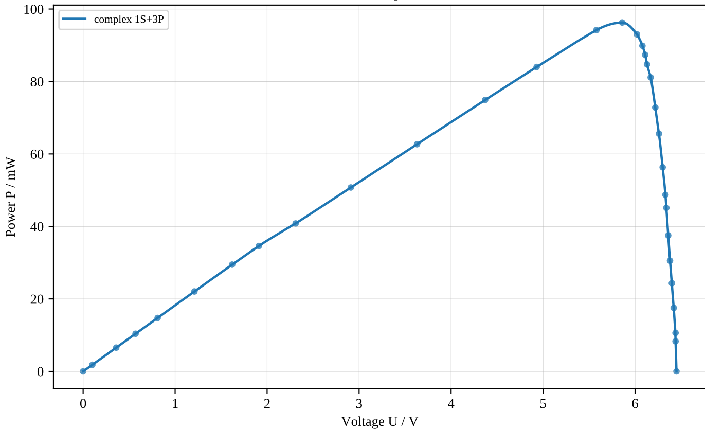
P-V curve: complex 1S+3P
