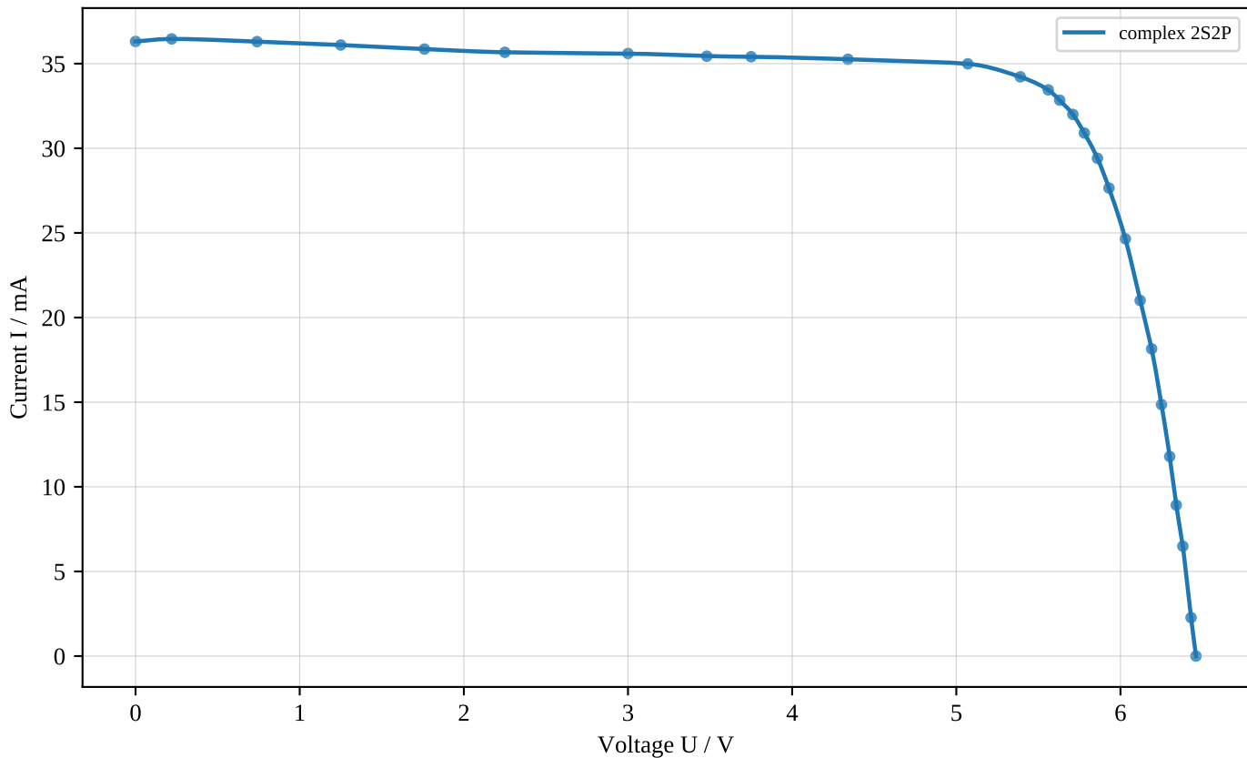
I-V curve: complex 2S2P
