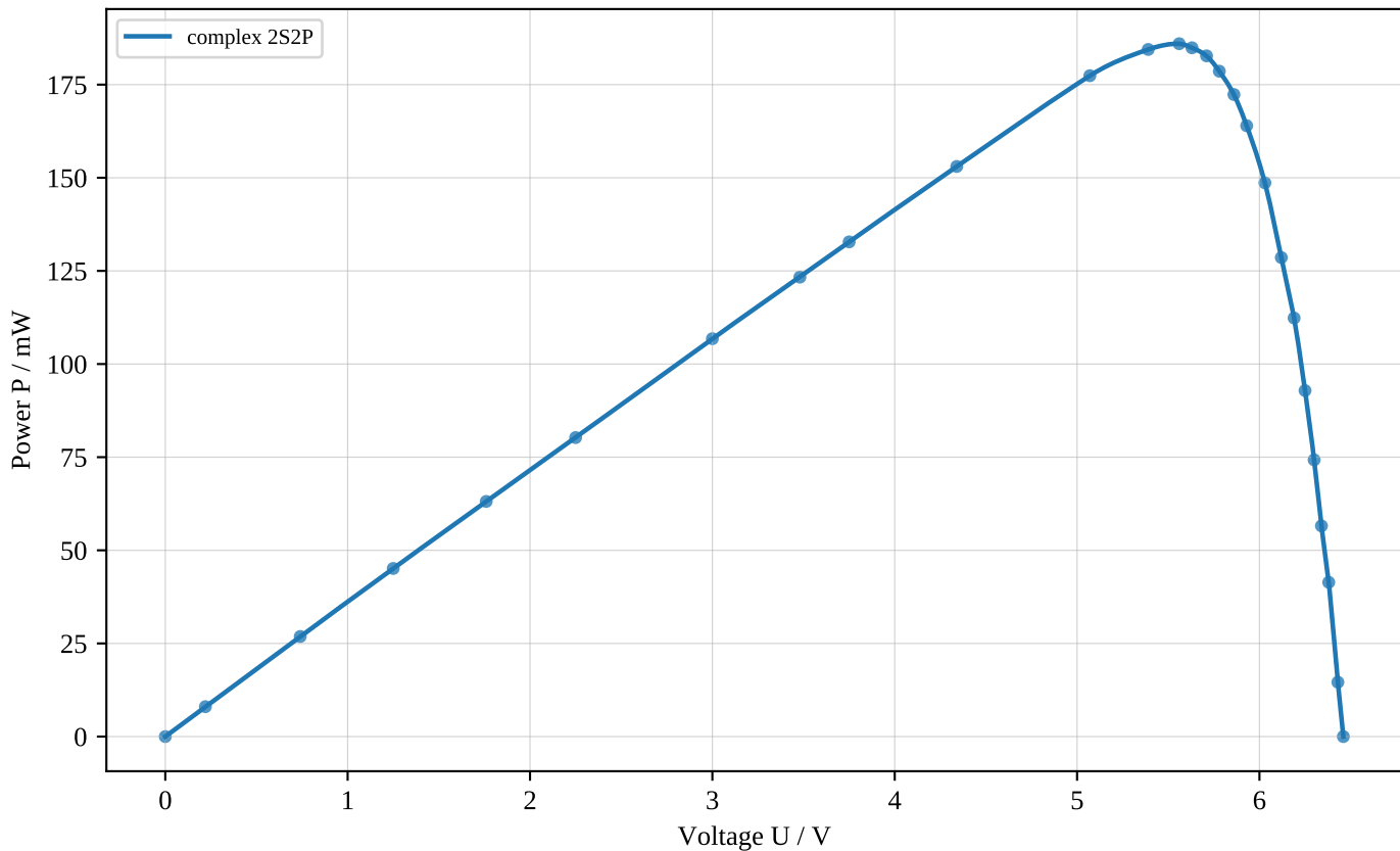
P-V curve: complex 2S2P
