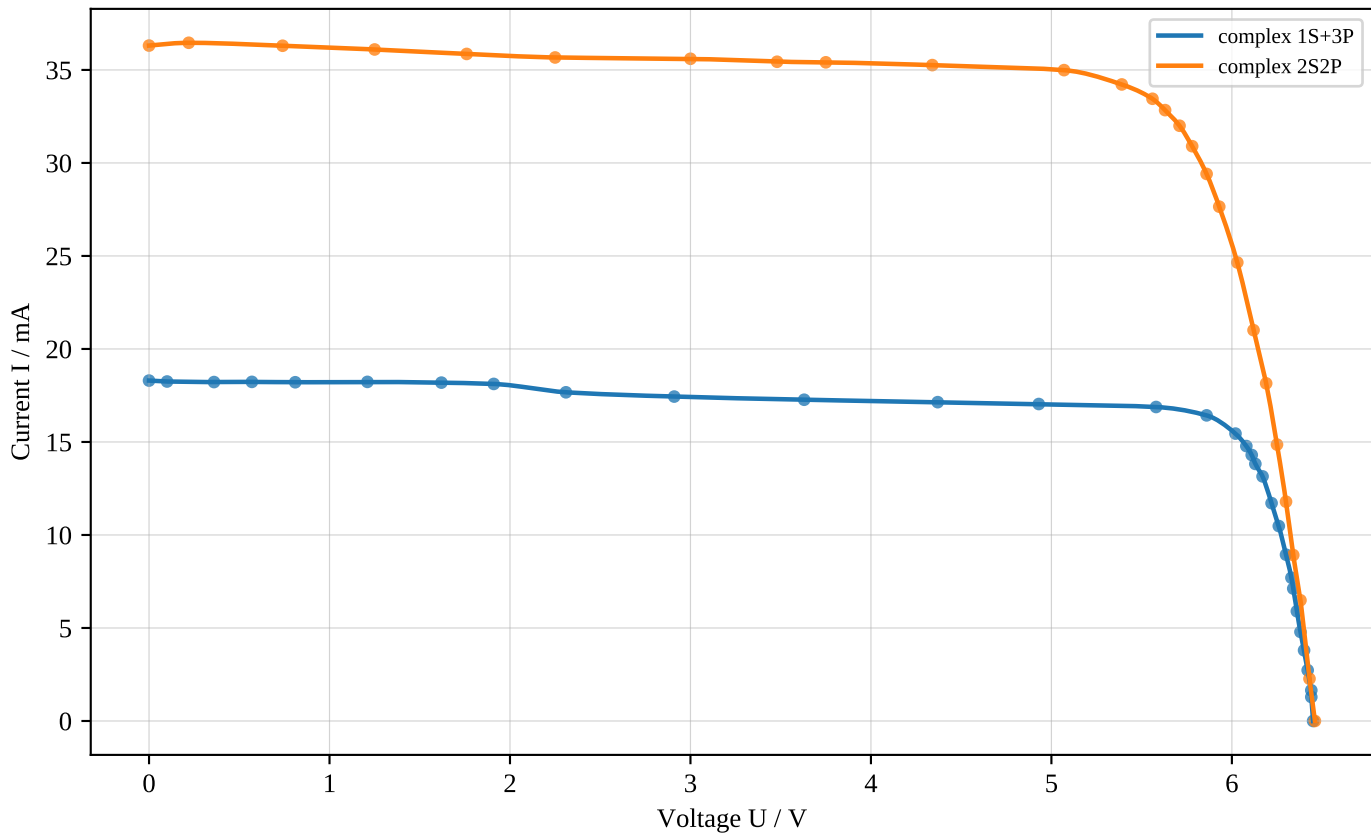
I-V curves: complex connections
