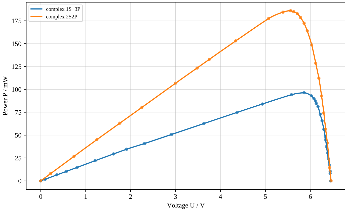
P-V curves: complex connections
