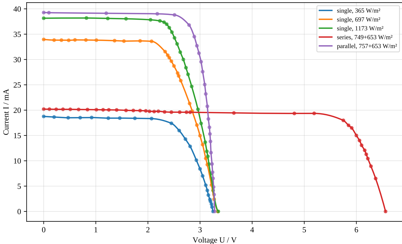
I-V curves: single cells, series and parallel
