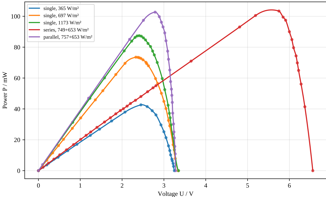
P-V curves: single cells, series and parallel
