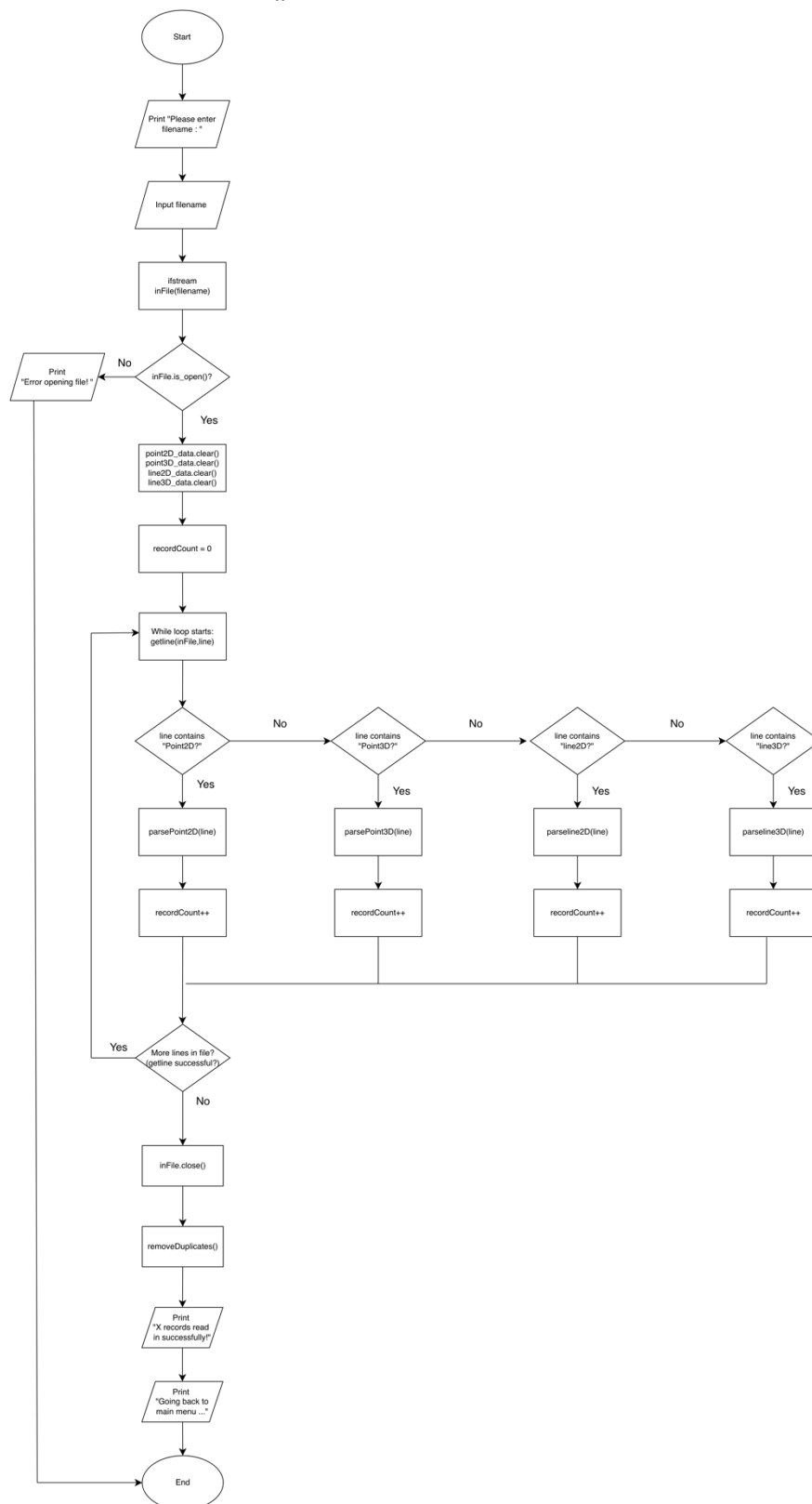
Flowchart 2: readData()
