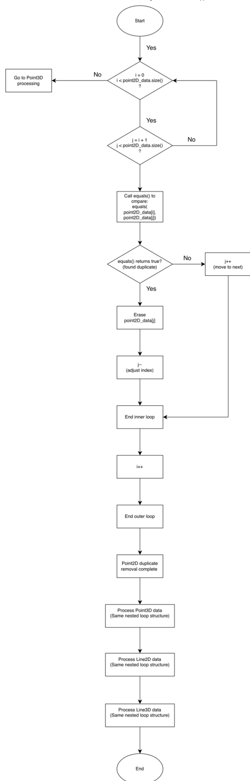
Flowchart 3: removeDuplicates()
