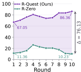
(b) Invalid Recall (%)
