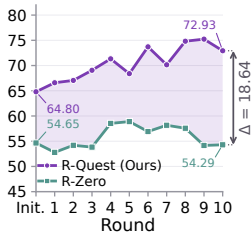
(a) Balanced Accuracy (%)
