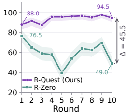
(c) Question Validity (%)
