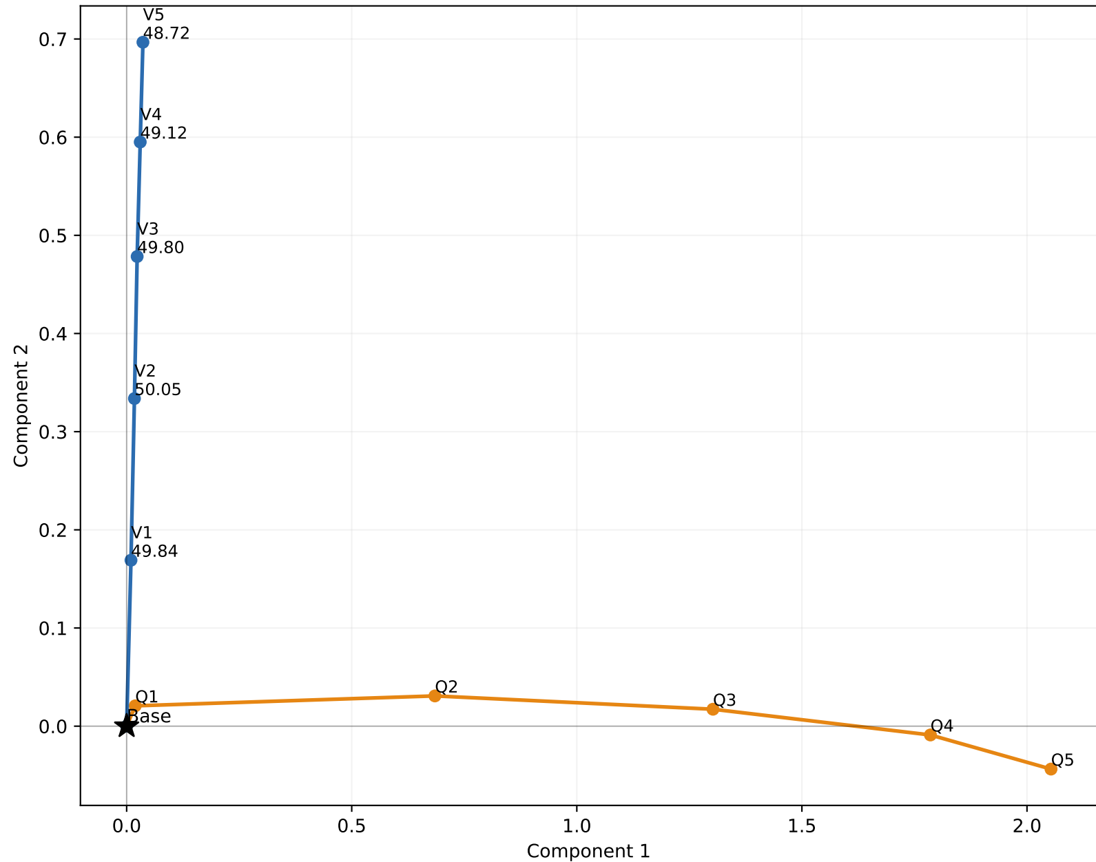
Cumulative Questioner and Rank1 Solver trajectories
