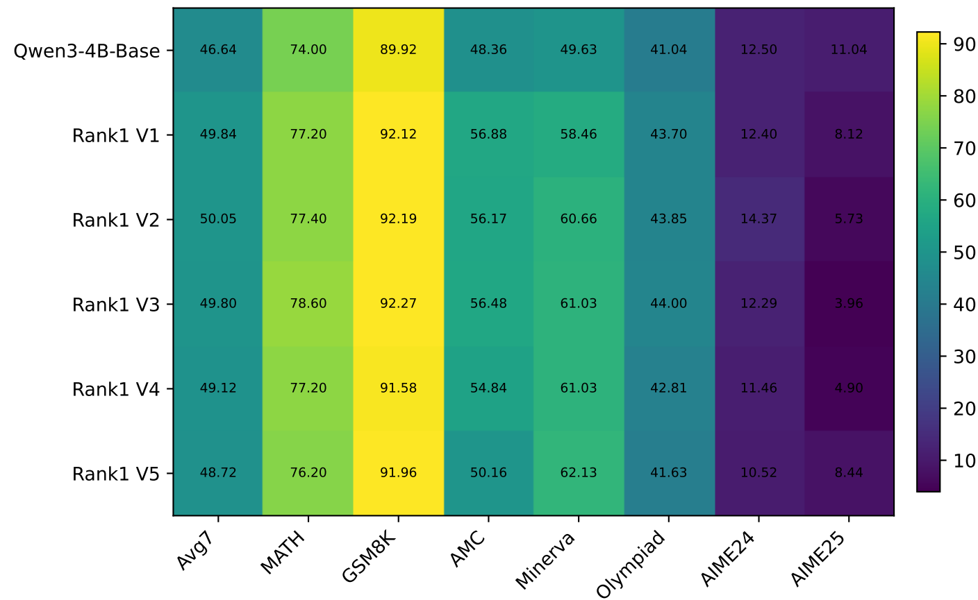
Evaluation scores
