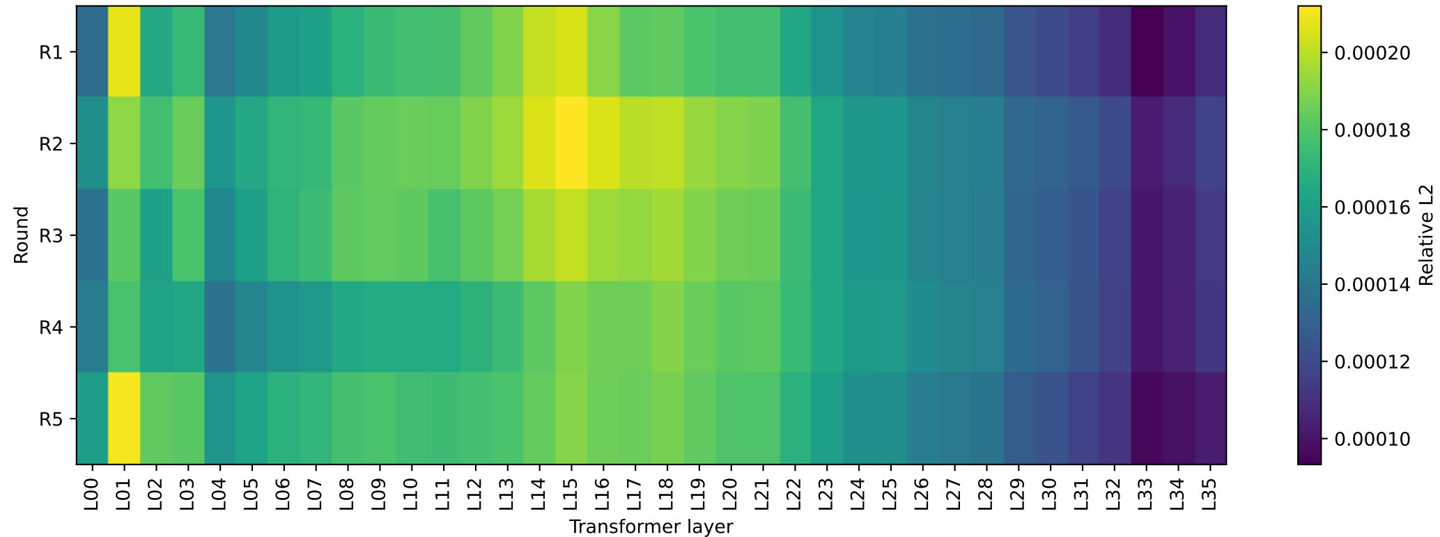
Per-layer relative delta norm: solver full
