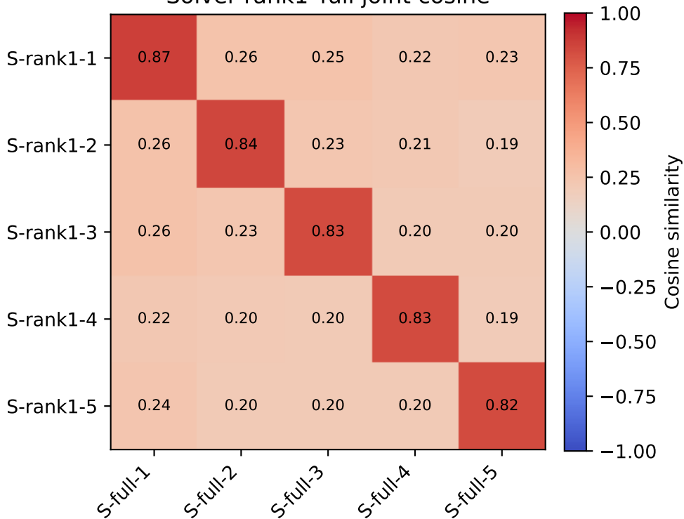
Solver rank1-full joint cosine
