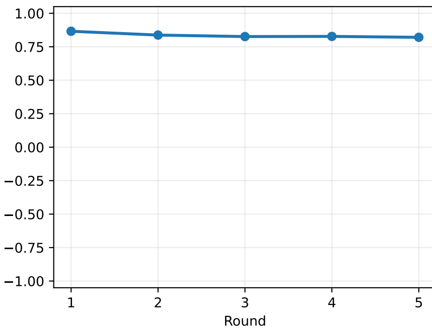
Rank1-Full cosine
