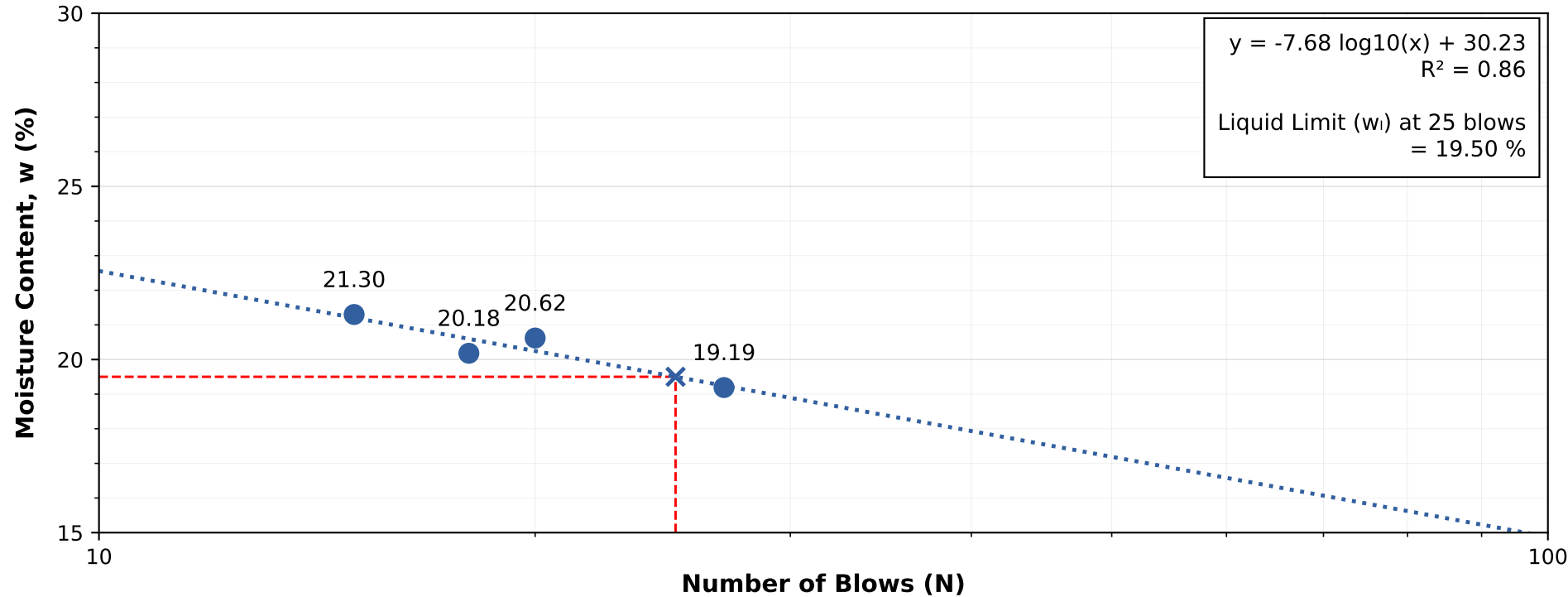
FLOW CURVE
