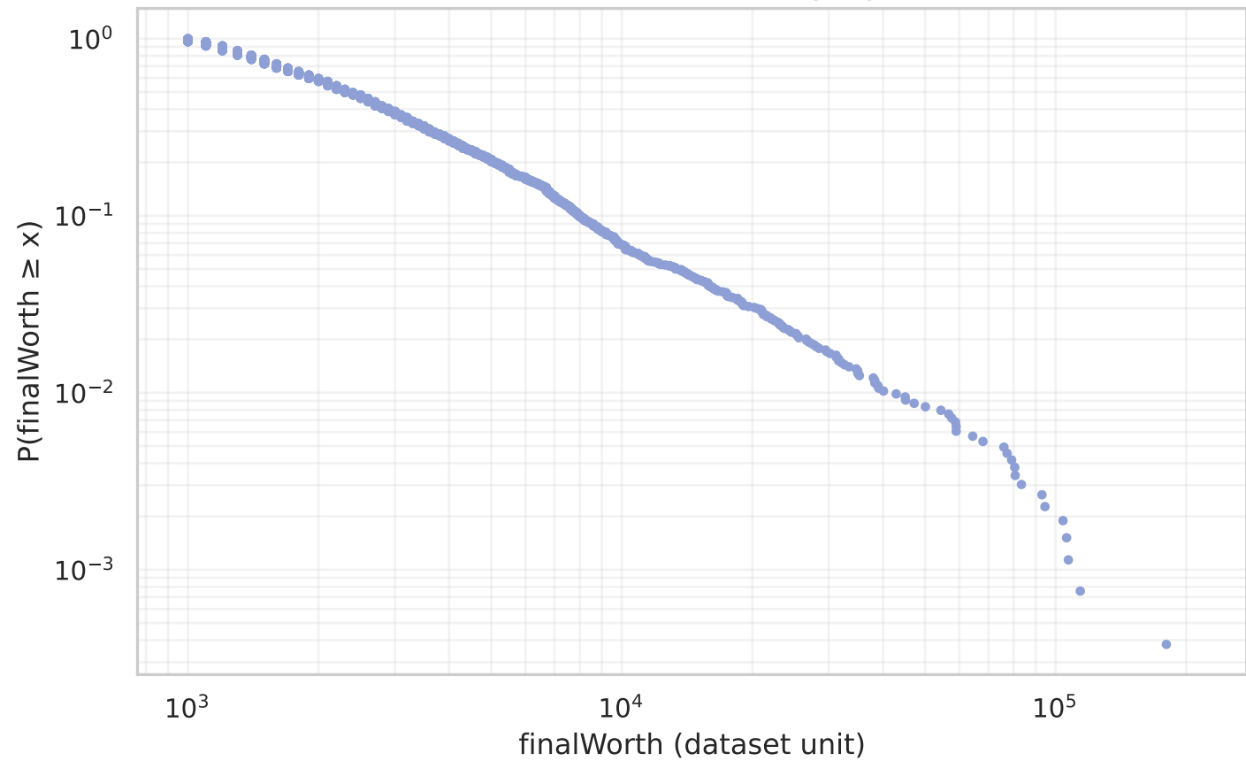
CCDF of finalWorth (log-log)
