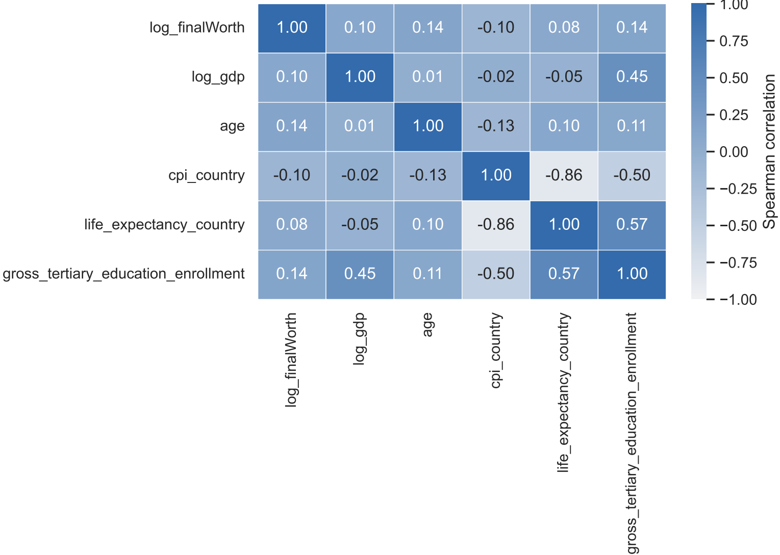
Spearman correlation heatmap (selected numeric features)
