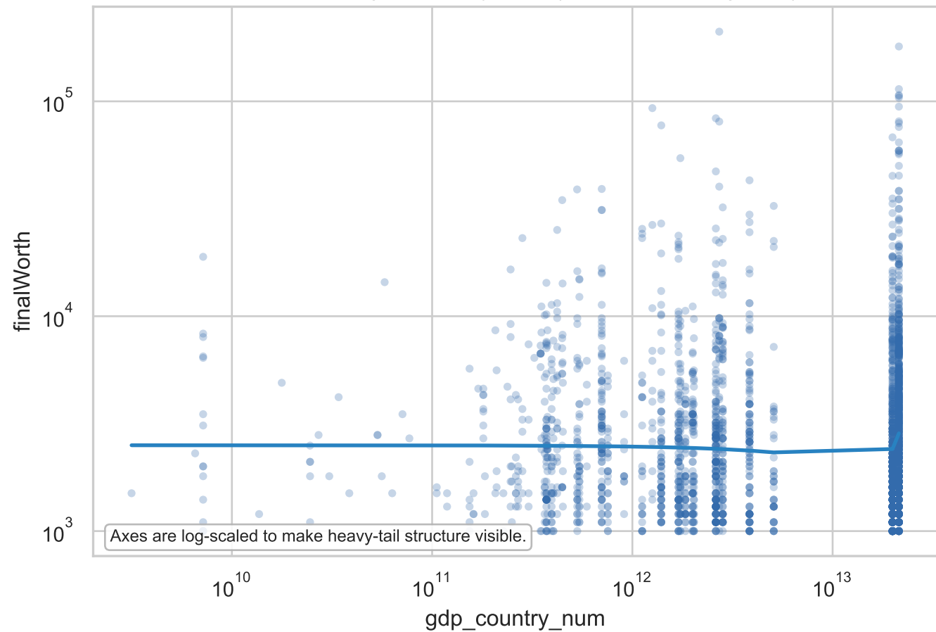
finalWorth vs gdp_country_num (raw variables; log axes)
