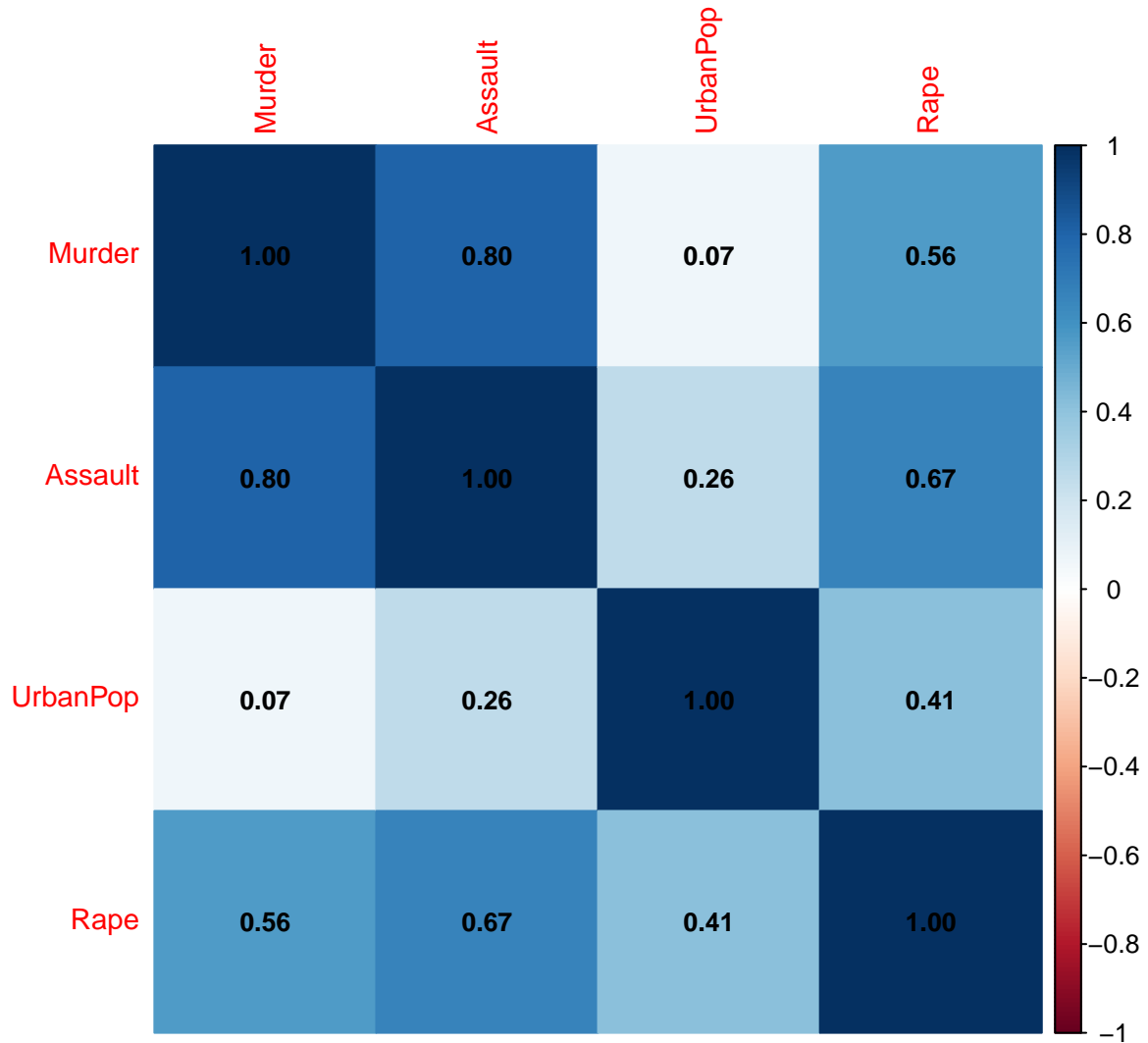
Correlation Matrix Heatmap: USArrests
