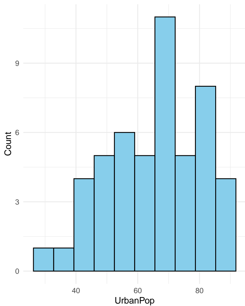
Histogram of UrbanPop (USArrests)
