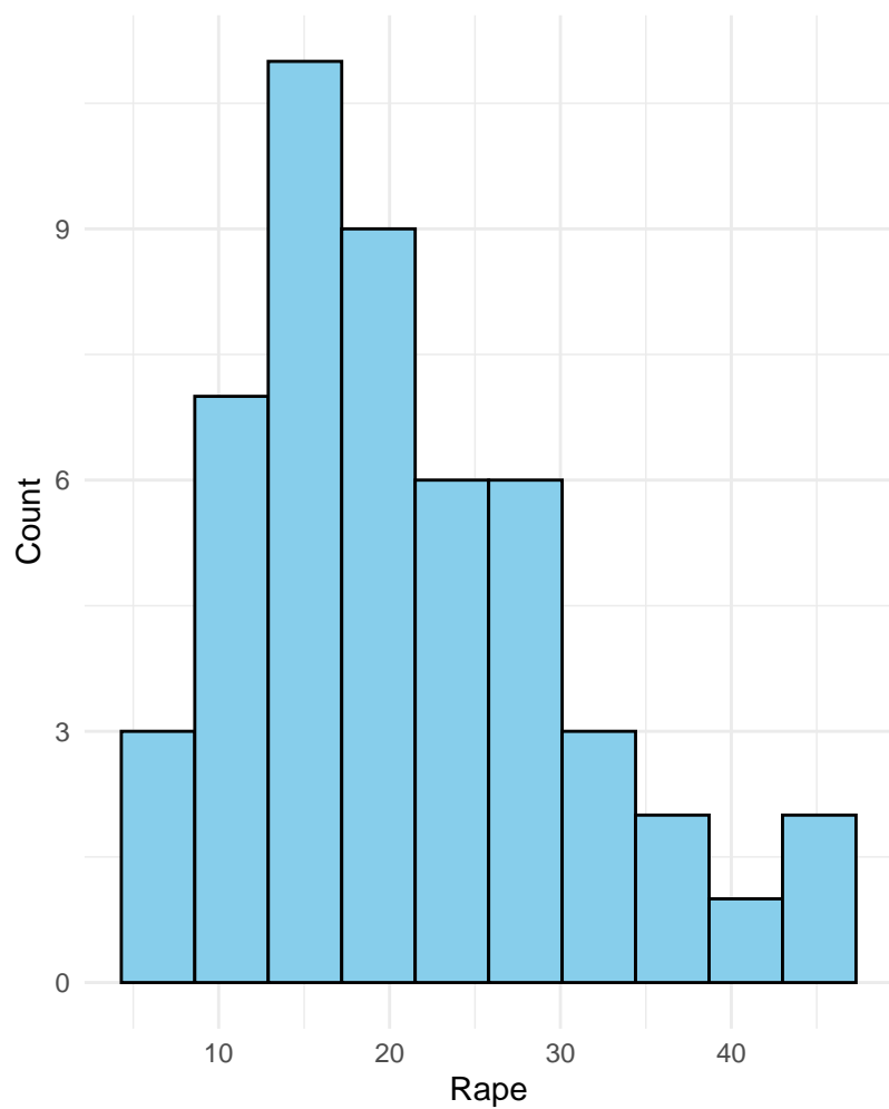
Histogram of Rape (USArrests)
