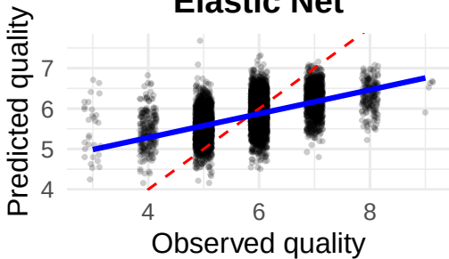
Elastic Net
