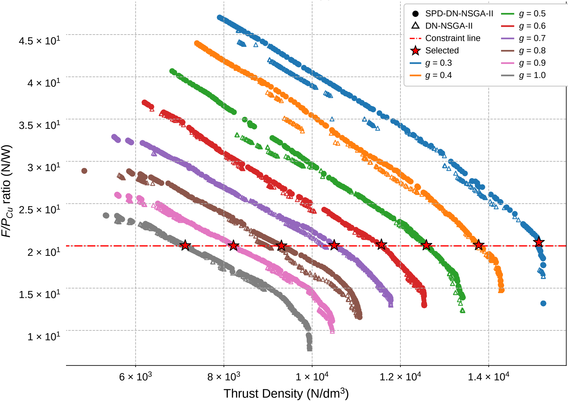
Pareto Front under Force-to-Copper-Loss Constraint
