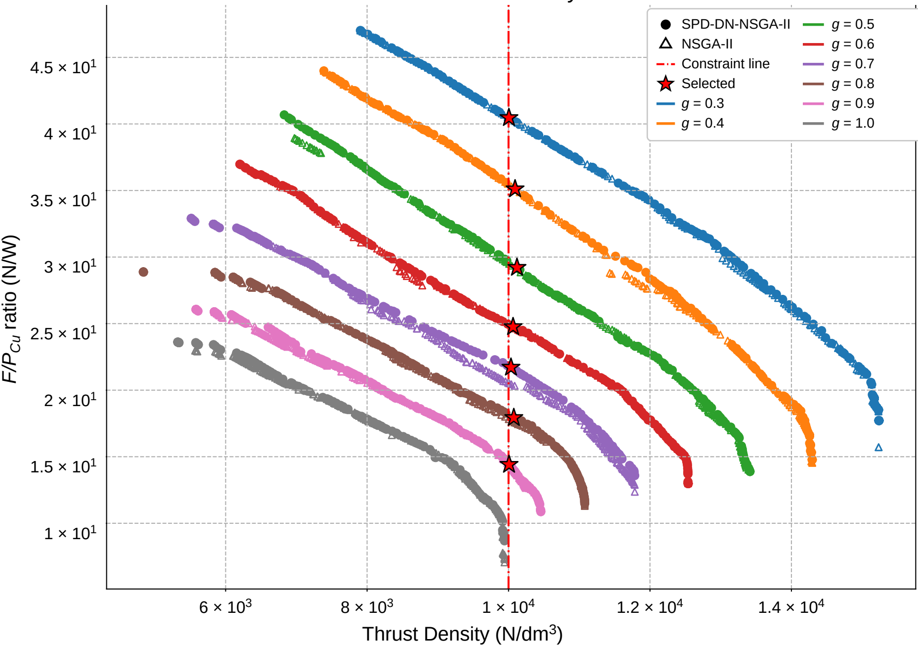
Pareto Front under Thrust-Density Constraint
