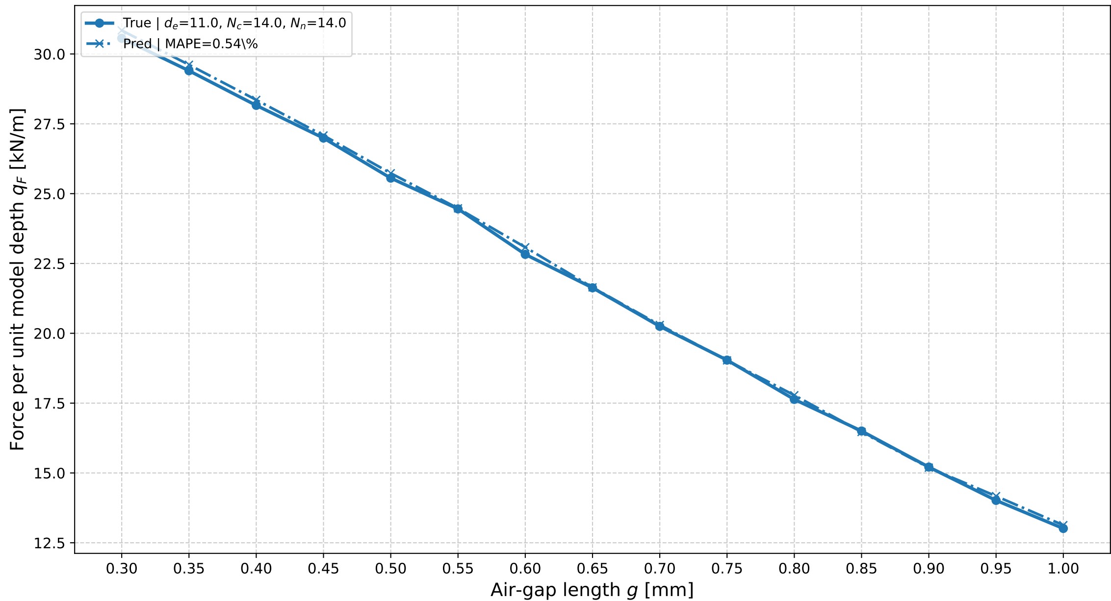
Comparison of Predicted and FEA Force-per-Unit-Depth Trend on g
