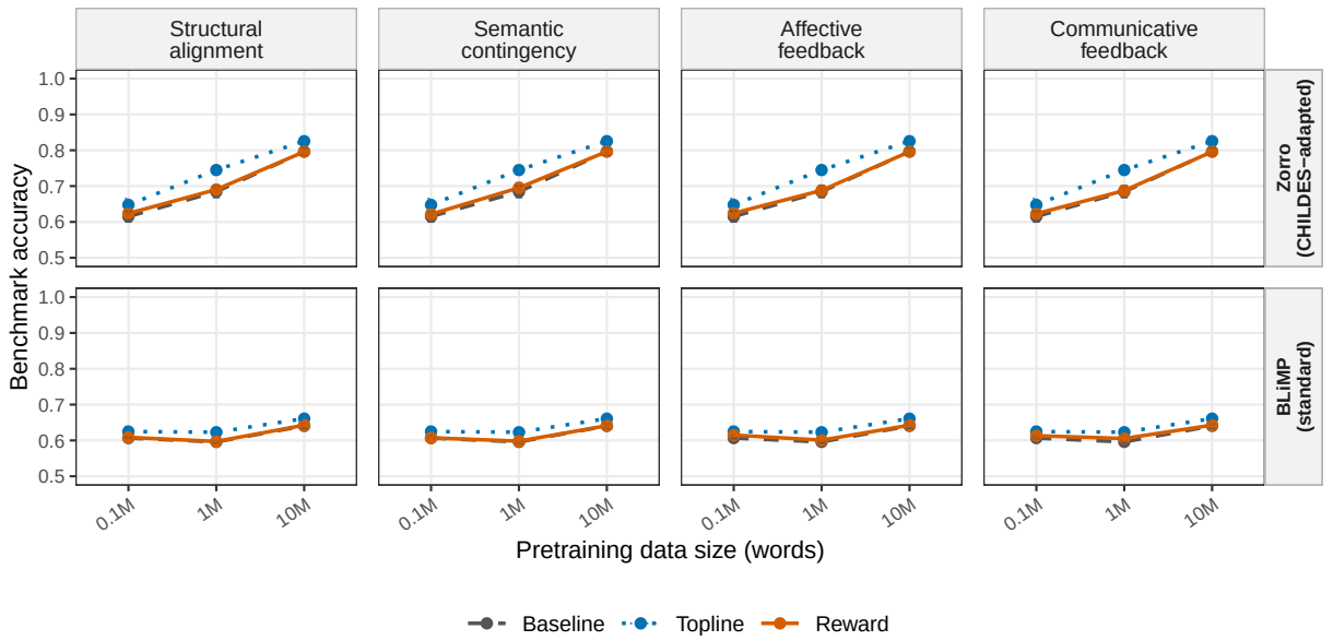
FIGURE 4.7 – Benchmark performance across pretraining scales for each reward family. Rows show Zorro and BLiMP minimal-pair accuracy; columns show the four empirical reward families. Within each panel, the baseline and topline trajectories are repeated to make the reward trajectory directly comparable at each scale. Means are computed over training seeds, after averaging over generation seeds. Error bars show \pm 1 standard deviation across independent units.
