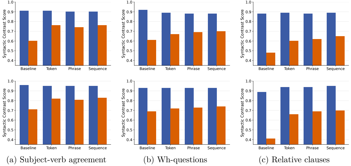
FIGURE 3.3 – Performance across retrieval granularities (token, phrase, sequence) in child-realistic (top row) and large-scale (bottom row) models ( k = 16, \tau = 3 ). Blue bars indicate high-frequency items and orange bars low-frequency items. Sequence-level retrieval is numerically the overall strongest, but the effect of retrieval granularity is overall small.
