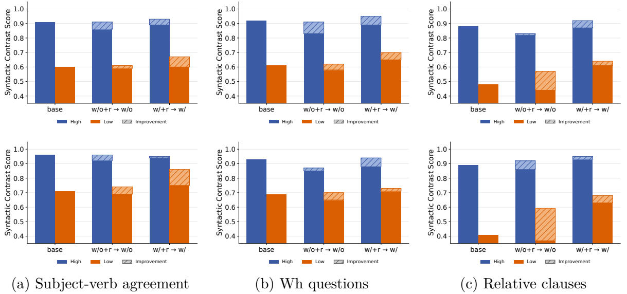
FIGURE 3.4 – Performance when retrieved sequences contain target syntactic structures (with) versus when they do not (without). Top row: child-scale model; bottom row: large-scale model ( k = 1 , \tau = 3 , sequence-level). Within each panel, the x -axis shows three conditions: base (no retrieval), w/o+r \rightarrow w/o (retrieval from a non-structural datastore, random vs. embedding-similarity), and w/+r \rightarrow w/ (retrieval from a structural datastore, random vs. embedding-similarity). Solid bars denote random retrieval (+r); hatched segments denote the additional gain from embedding-similarity retrieval over random. Blue and orange bars correspond to high- and low-frequency items, respectively. Random retrieval baselines isolate the contribution of structural match in the datastore from semantic ranking by the retriever.
