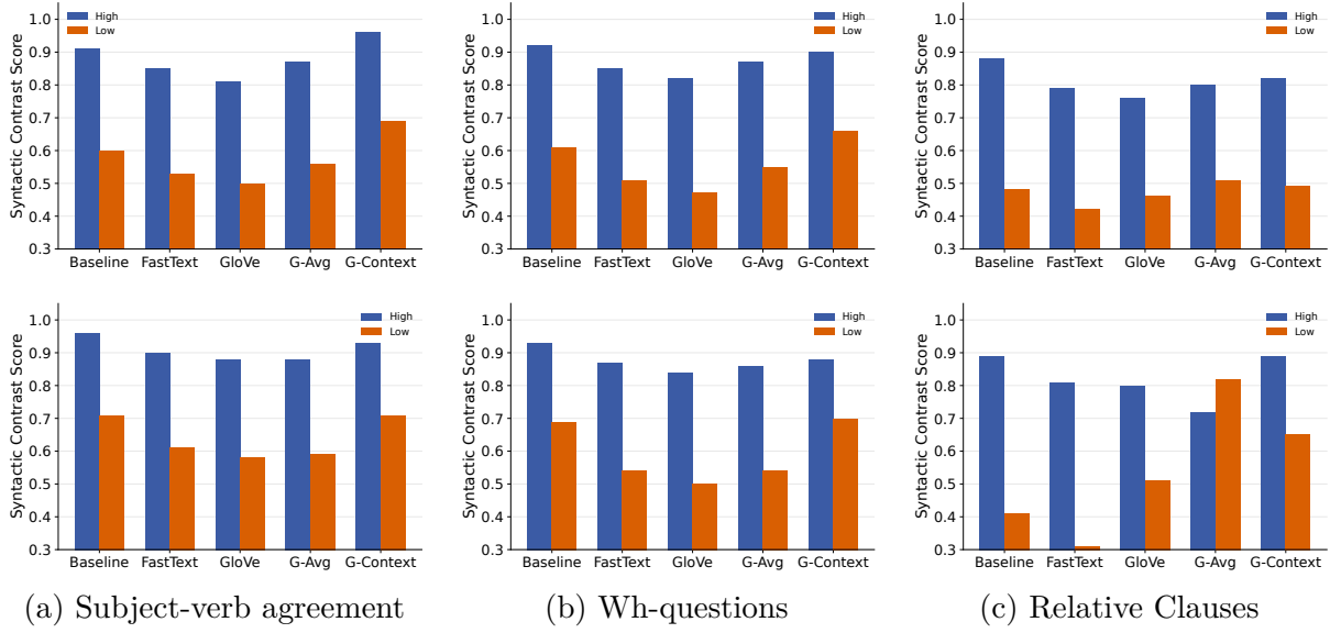
FIGURE 3.3 – Performance on syntactic contrasts using semantics-only retrieval strategies compared to full retrieval ( k = 1 , \tau = 3 ) of the child-realistic (top row) and large-scale (bottom row) models. Blue bars indicate high-frequency items and orange bars low-frequency items. We report the token-level retrieval here.
