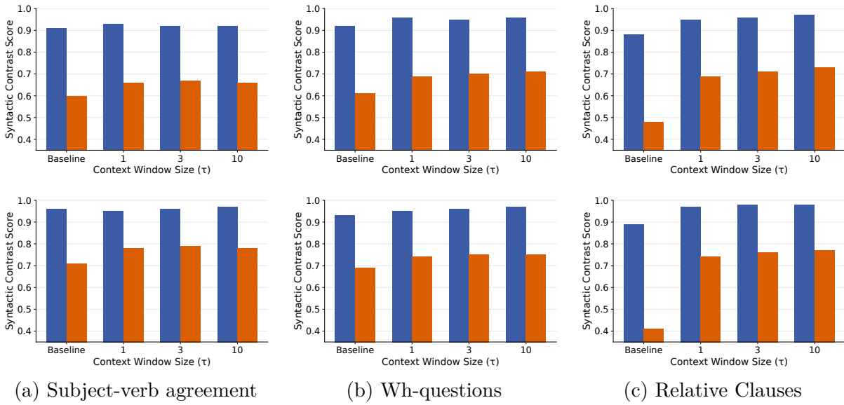
FIGURE 3.6 – Performance across different context windows of the child-realistic (top row) and large-scale (bottom row) models. Blue bars indicate high-frequency items and orange bars low-frequency items. We report the sequence-level retrieval given that it yields the best test performance. Overall, larger context windows ( \tau = 10 ) tend to yield stronger performance, especially for structurally complex phenomena, whereas simpler dependencies are less sensitive to context size.
