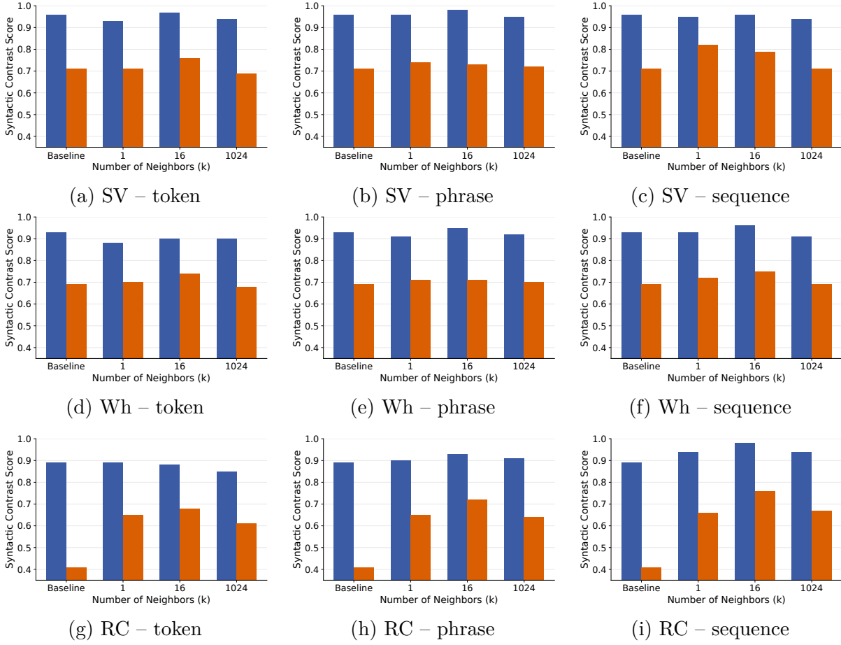
FIGURE 3.13 – Effect of number of retrieved neighbors ( k \in \{1, 16, 1024\} ) for GPT-2 XL at \tau = 3 . Results are consistent with \tau = 1 (Figure 3.12): k = 16 provides the best balance between evidence aggregation and noise across phenomena and frequency bands.
