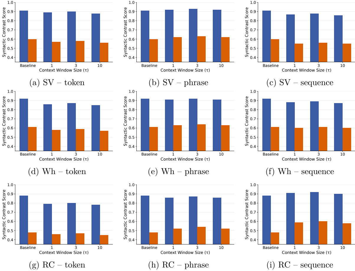
FIGURE 3.11 – Effect of context window size ( \tau \in \{1, 3, 10\} ) for the child-realistic model at k = 1024 . Performance degradation at large k is more pronounced than for GPT-2 XL, particularly for low-frequency RCs, suggesting the smaller model is more susceptible to retrieval noise.
