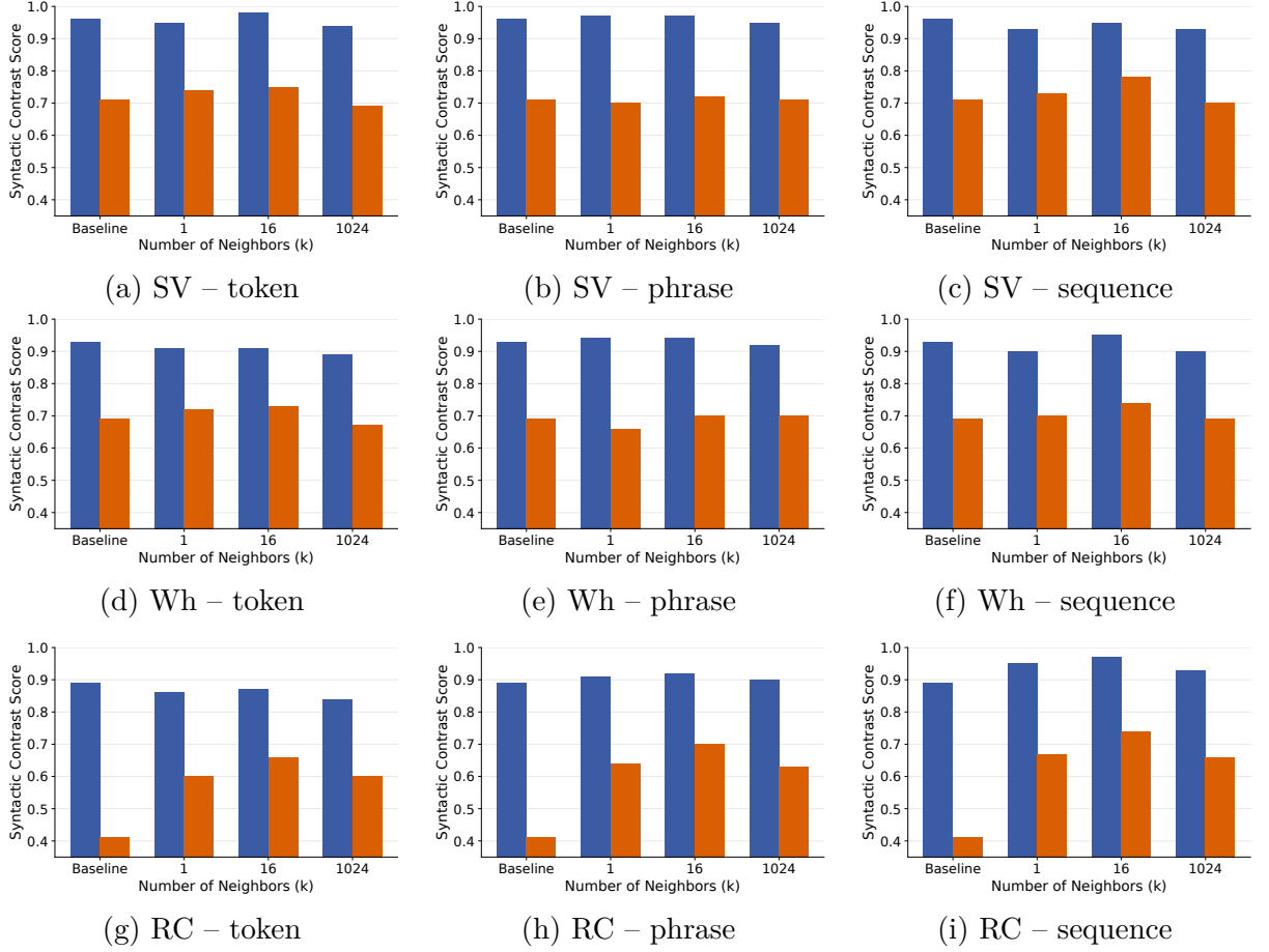
FIGURE 3.12 – Effect of number of retrieved neighbors ( k \in \{1, 16, 1024\} ) for GPT-2 XL at \tau = 1 . The non-monotonic pattern holds: k = 16 outperforms both k = 1 and k = 1024 across most conditions, with degradation at large k most severe for sequence-level retrieval and low-frequency items.
