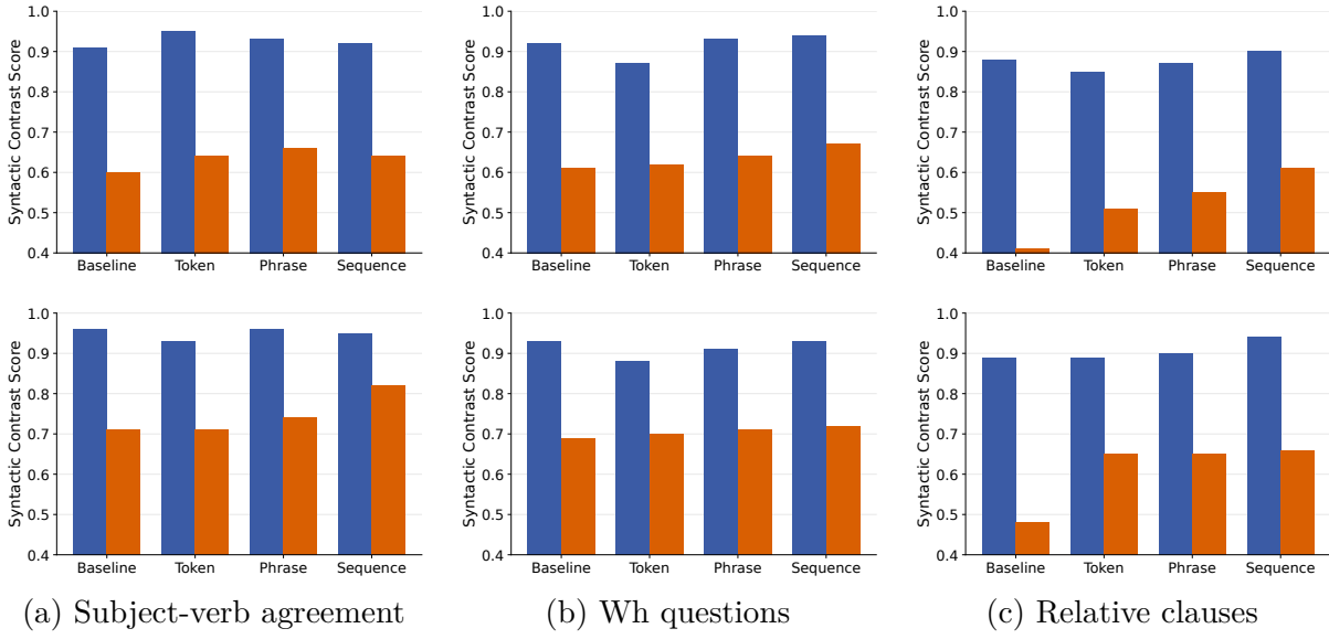
FIGURE 3.5 – Performance across retrieval granularities (token, phrase, sequence) in child-realistic (top row) and large-scale (bottom row) models ( k = 1 , \tau = 3 ). Blue bars indicate high-frequency items and orange bars low-frequency items. Optimal granularity varies by phenomenon and frequency: sequence-level retrieval generally performs best for low-frequency items in wh-questions and relative clauses, while patterns for subject-verb agreement vary by model scale.
