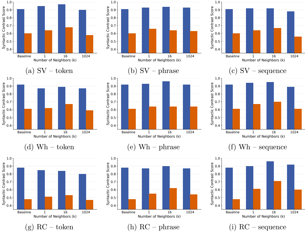
FIGURE 3.15 – Effect of number of retrieved neighbors ( k \in \{1, 16, 1024\} ) for the child-realistic model at \tau = 3 . Consistent with all other configurations, k = 16 provides the best balance between evidence aggregation and noise, with gains most pronounced for low-frequency RCs and Wh-questions.
