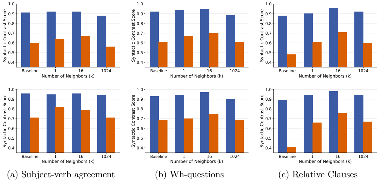
FIGURE 3.7 – Performance across different numbers of retrieved neighbors of the child-realistic (top row) and large-scale (bottom row) models. Blue bars indicate high-frequency items and orange bars low-frequency items. We report the sequence-level retrieval given that it yields the best test performance. Performance exhibits a non-monotonic pattern: increasing the number of neighbors from k = 1 to a moderate value ( k = 16 ) generally improves performance across phenomena and frequency bands, while further increasing to large values ( k = 1024 ) leads to degradation.
