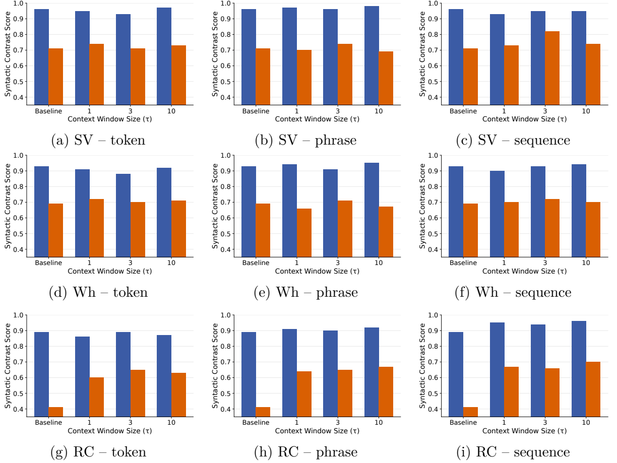
FIGURE 3.8 – Effect of context window size ( \tau \in \{1, 3, 10\} ) for GPT-2 XL at k = 1 . Larger context windows benefit low-frequency items more than high-frequency items, particularly for sequence-level retrieval and structurally complex phenomena (Wh, RCs). Subject-verb agreement is less sensitive to context size.
