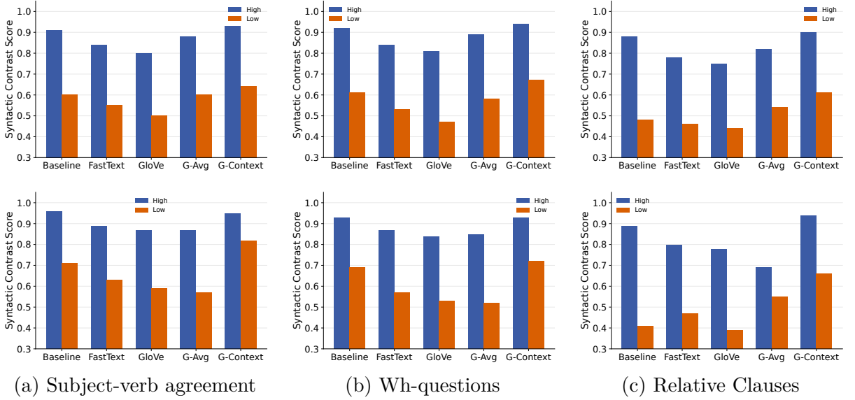
FIGURE 3.1 – Performance on syntactic contrasts using semantics-only retrieval strategies compared to full retrieval ( k = 1 , \tau = 3 ) of the child-realistic (top row) and large-scale (bottom row) models. Blue bars indicate high-frequency items and orange bars low-frequency items. We report the sequence-level retrieval given that it yields the best test performance.
