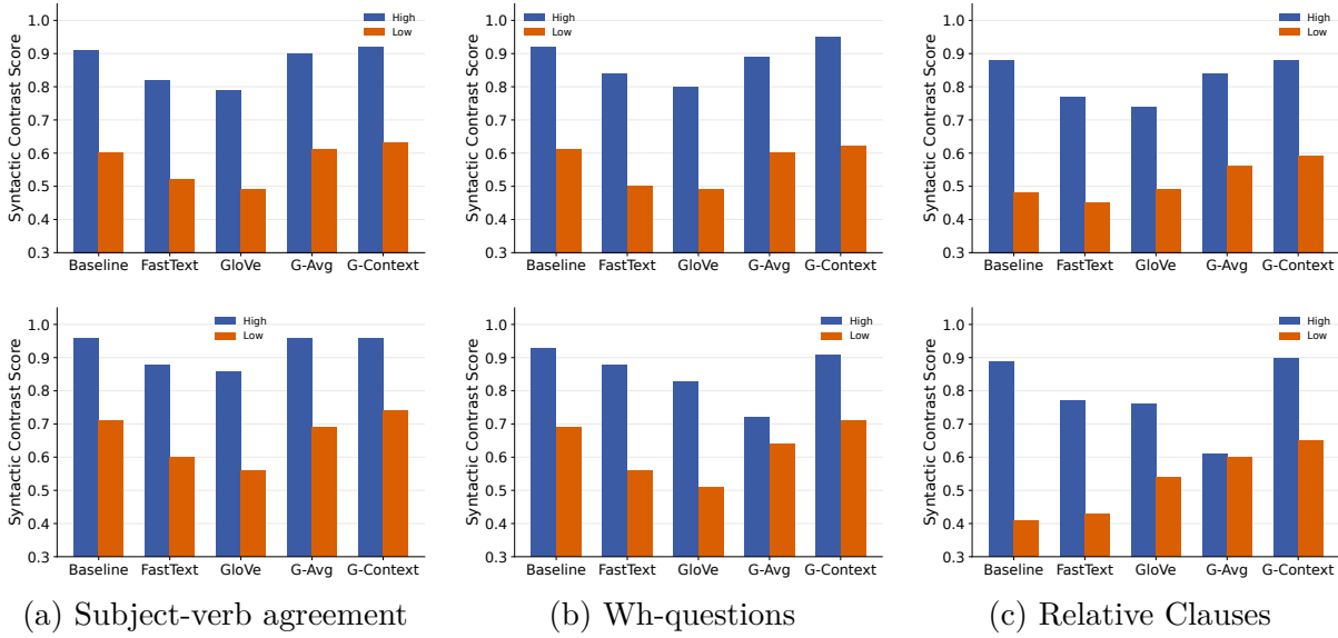
FIGURE 3.2 – Performance on syntactic contrasts using semantics-only retrieval strategies compared to full retrieval ( k = 1 , \tau = 3 ) of the child-realistic (top row) and large-scale (bottom row) models. Blue bars indicate high-frequency items and orange bars low-frequency items. We report the phrase-level retrieval here.
