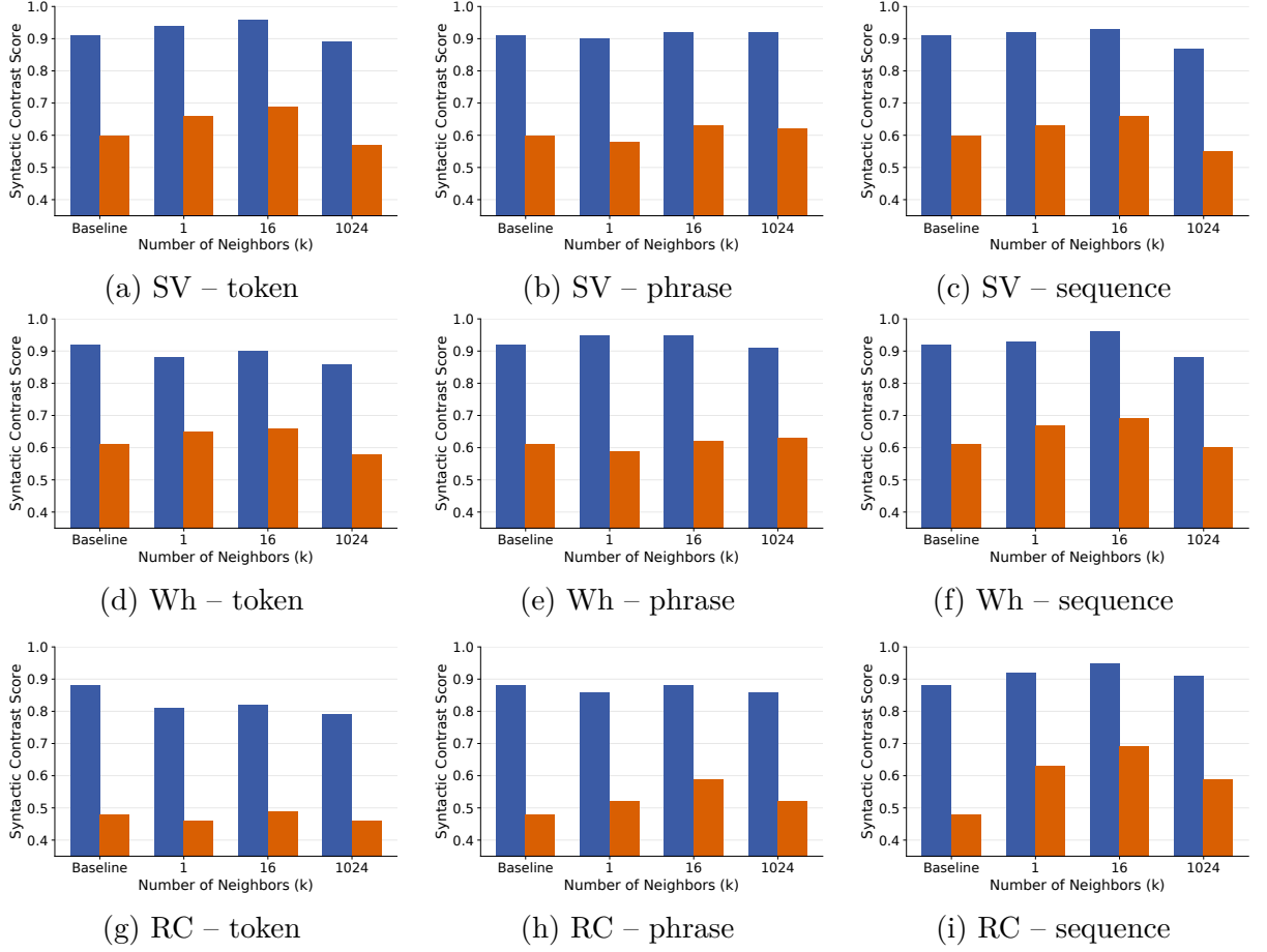
FIGURE 3.14 – Effect of number of retrieved neighbors ( k \in \{1, 16, 1024\} ) for the child-realistic model at \tau = 1 . The non-monotonic pattern holds across both model scales, with k = 16 providing the best overall performance and k = 1024 degrading most severely for low-frequency RCs.
