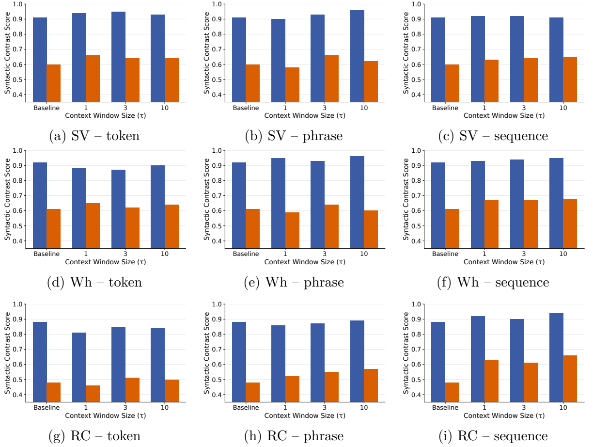
Figure 4.8 – Effect of context window size ( \tau \in \{1, 3, 10\} ) for the child-realistic model at k = 1 . Blue bars indicate high-frequency items and orange bars indicate low-frequency items; baseline results are shown for reference.
