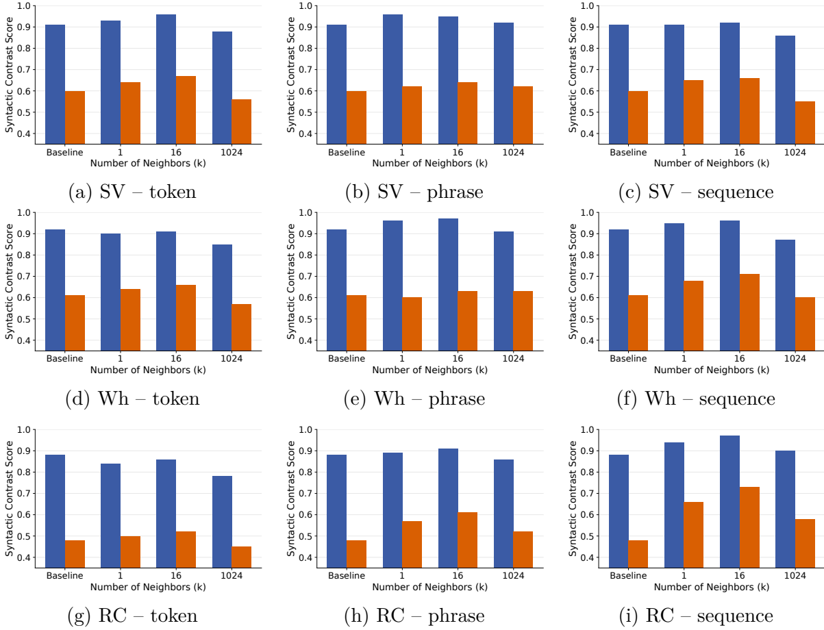
Figure 4.13 – Effect of number of retrieved neighbors ( k \in \{1, 16, 1024\} ) for the child-realistic model at \tau = 10 . Blue bars indicate high-frequency items and orange bars indicate low-frequency items; baseline results are shown for reference.
