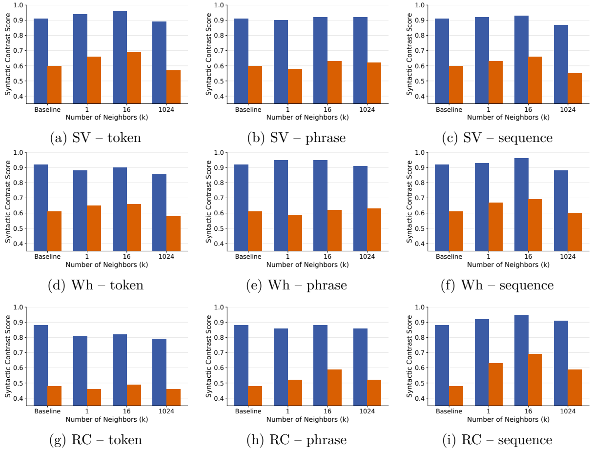
Figure 4.12 – Effect of number of retrieved neighbors ( k \in \{1, 16, 1024\} ) for the child-realistic model at \tau = 1 . Blue bars indicate high-frequency items and orange bars indicate low-frequency items; baseline results are shown for reference.
