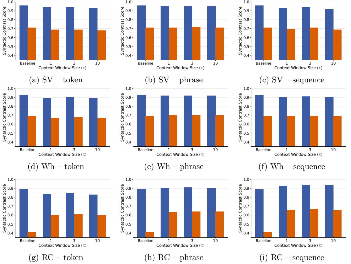
FIGURE 3.7 – Effect of context window size ( \tau \in \{1, 3, 10\} ) for GPT-2 XL at k = 1024 . Blue bars indicate high-frequency items and orange bars indicate low-frequency items; baseline results are shown for reference.
