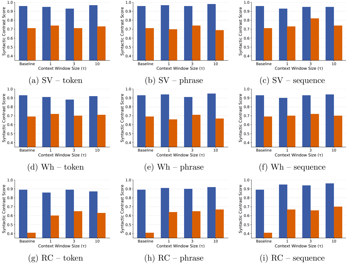
FIGURE 3.6 – Effect of context window size ( \tau \in \{1, 3, 10\} ) for GPT-2 XL at k = 1 . Blue bars indicate high-frequency items and orange bars indicate low-frequency items; baseline results are shown for reference.
