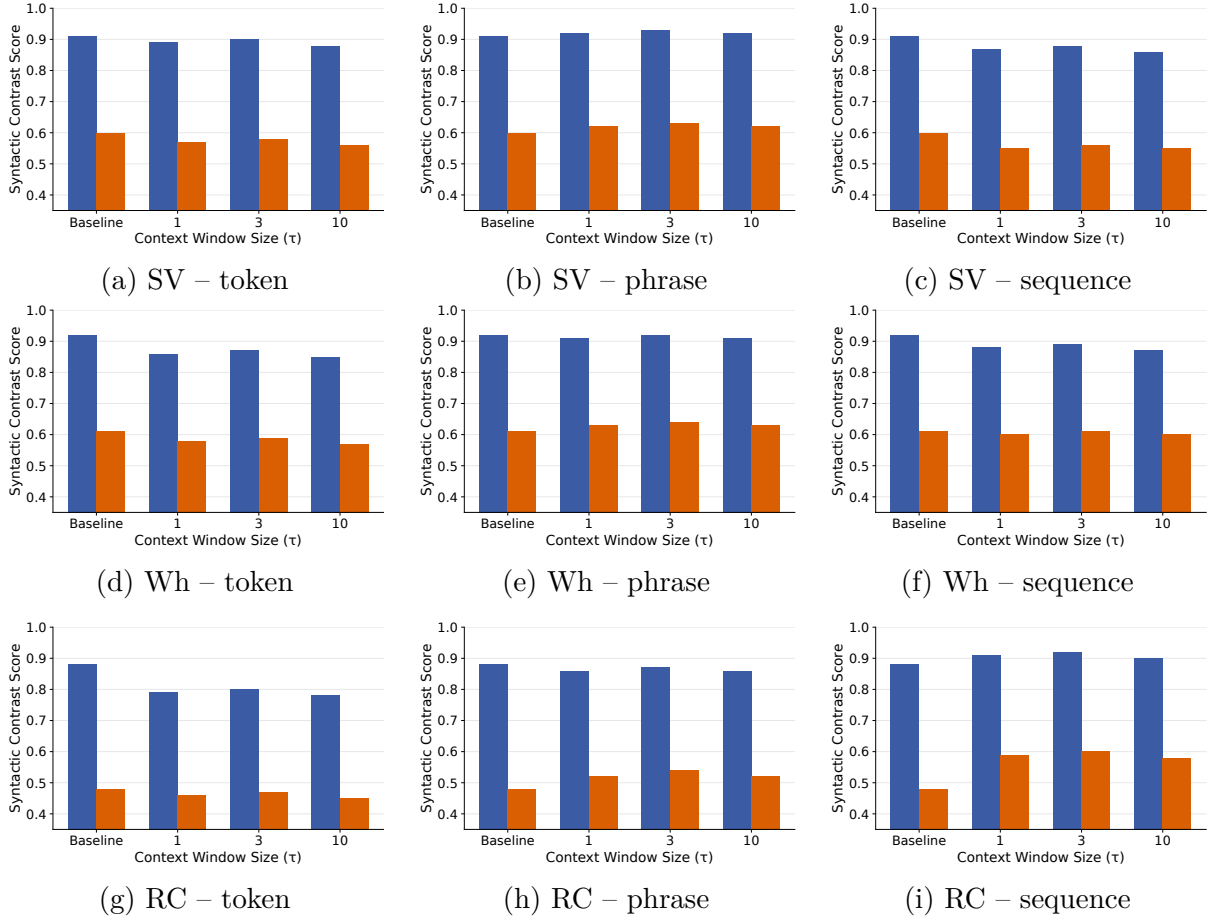
FIGURE 3.9 – Effect of context window size ( \tau \in \{1, 3, 10\} ) for the child-realistic model at k = 1024 . Blue bars indicate high-frequency items and orange bars indicate low-frequency items; baseline results are shown for reference.
