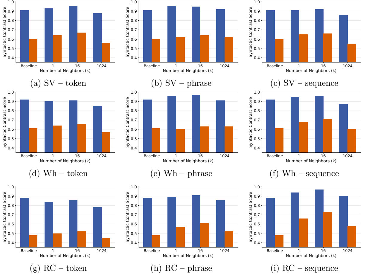
FIGURE 3.13 – Effect of number of retrieved neighbors ( k \in \{1, 16, 1024\} ) for the child-realistic model at \tau = 10 . Blue bars indicate high-frequency items and orange bars indicate low-frequency items; baseline results are shown for reference.
