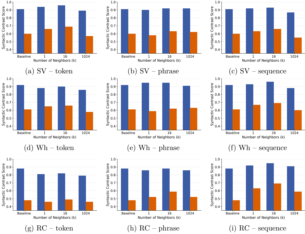
FIGURE 3.12 – Effect of number of retrieved neighbors ( k \in \{1, 16, 1024\} ) for the child-realistic model at \tau = 1 . Blue bars indicate high-frequency items and orange bars indicate low-frequency items; baseline results are shown for reference.
