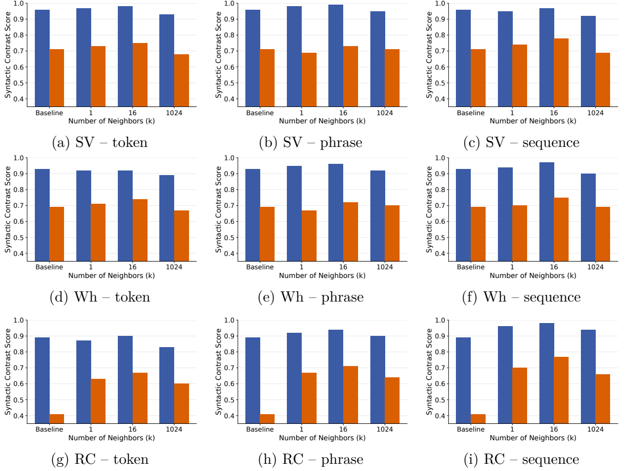
FIGURE 3.11 – Effect of number of retrieved neighbors ( k \in \{1, 16, 1024\} ) for GPT-2 XL at \tau = 10 . Blue bars indicate high-frequency items and orange bars indicate low-frequency items; baseline results are shown for reference.
