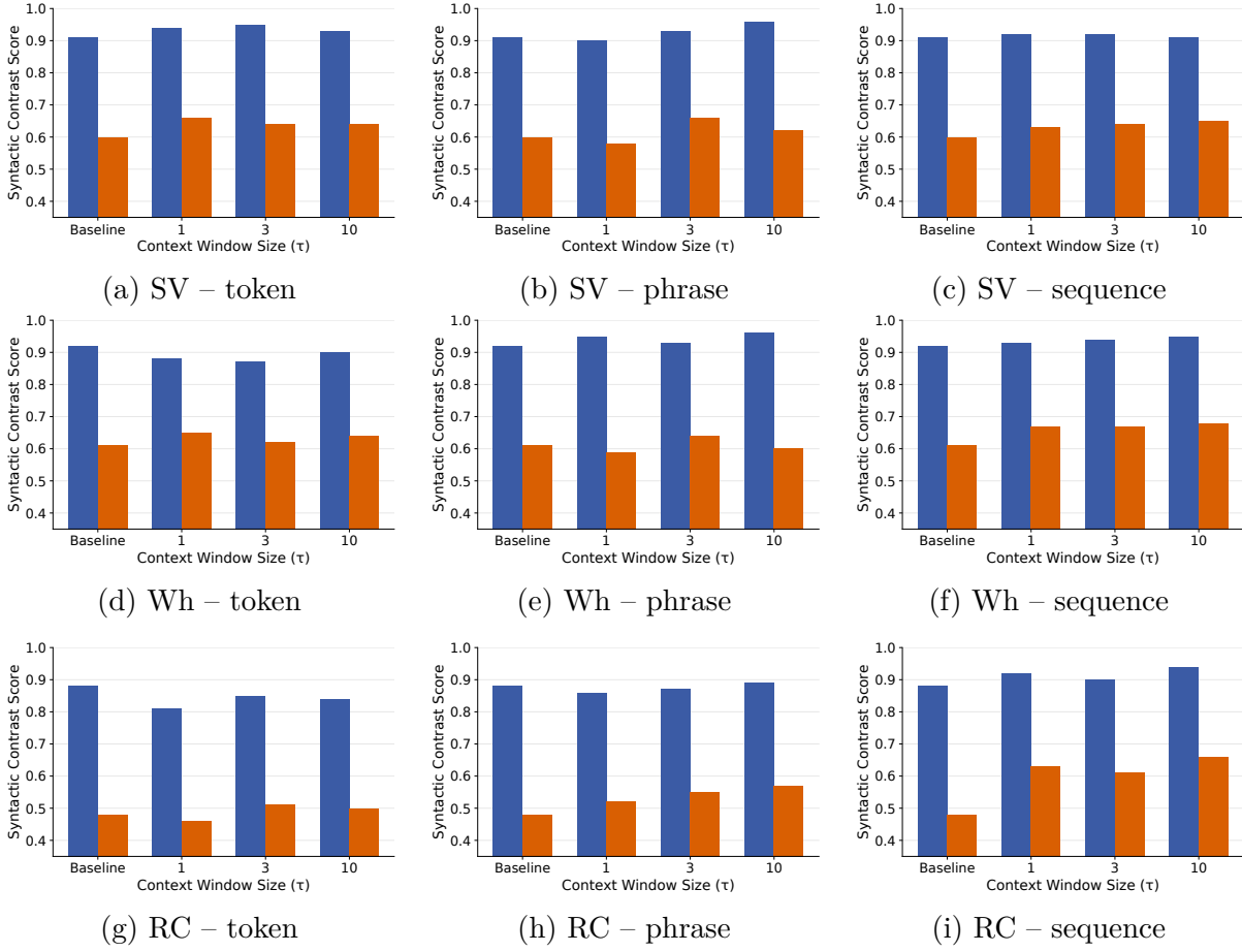
FIGURE 3.8 – Effect of context window size ( \tau \in \{1, 3, 10\} ) for the child-realistic model at k = 1 . Blue bars indicate high-frequency items and orange bars indicate low-frequency items; baseline results are shown for reference.
