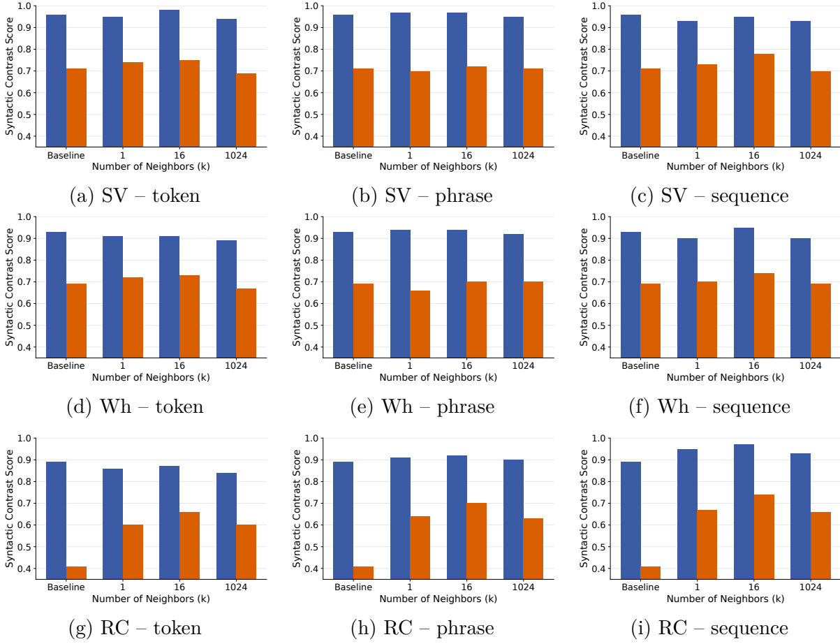
FIGURE 3.10 – Effect of number of retrieved neighbors ( k \in \{1, 16, 1024\} ) for GPT-2 XL at \tau = 1 . Blue bars indicate high-frequency items and orange bars indicate low-frequency items; baseline results are shown for reference.
