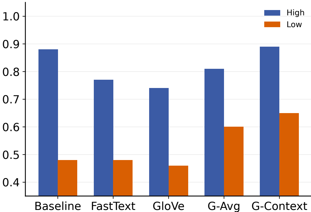
Syntactic Contrast Score
